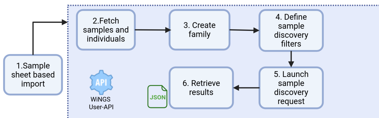
Fig. S4. SV sample discovery Workflow
