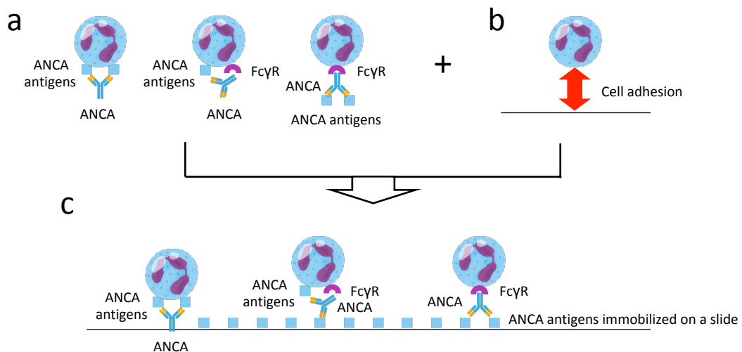
Figure S2. Concept of in vitro assay.
