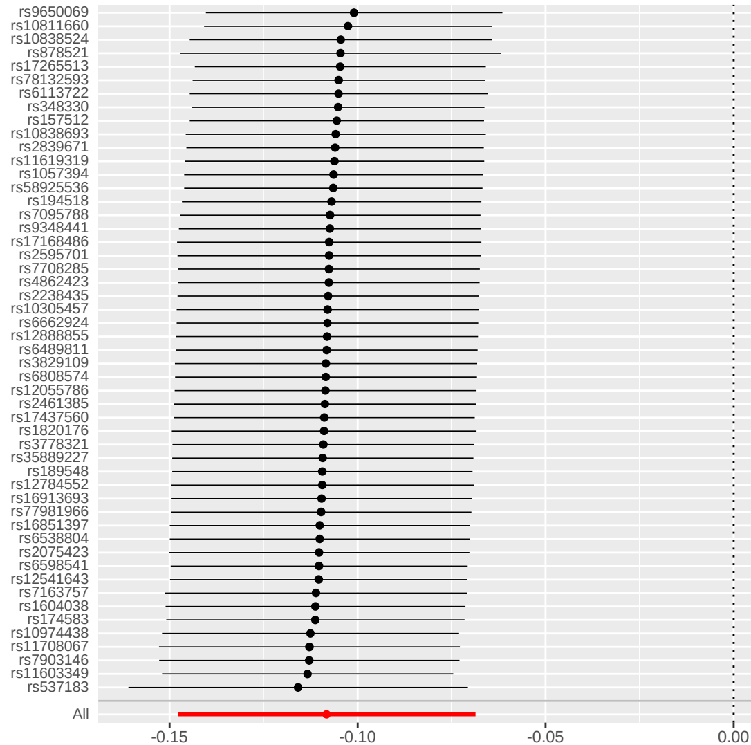
MR leave-one-out sensitivity analysis for 'exposure' on 'Serum 25-Hydroxyvitamin D levels || id:ebi-a-GCST90000618'
