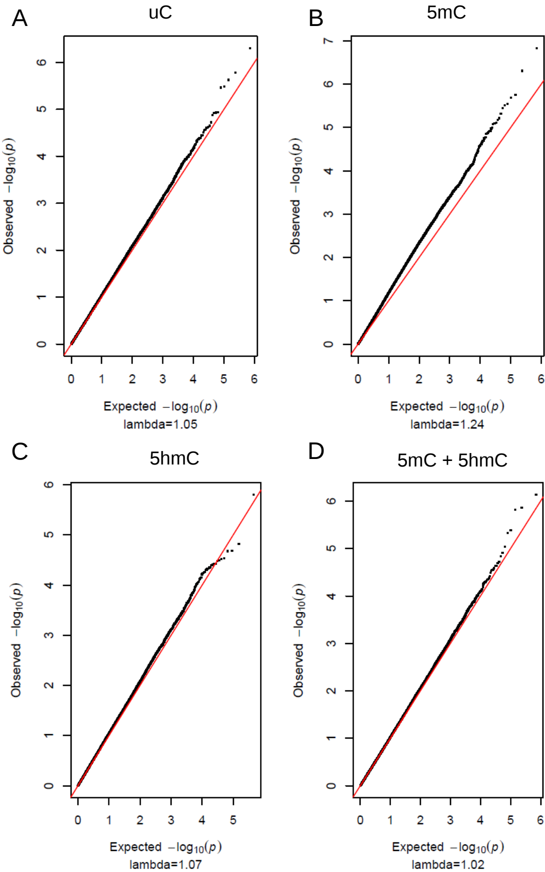
Figure S1 Quantile-quantile (Q-Q) plots of expected versus observed P value to check for inflation in linear regression analyses. Q-Q plots are shown for (A) unmodified cytosine (uC) (1-BS data), (B) 5mC (OxBS data), (C) 5hmC (BS – OxBS data) and (D) total DNA modifications (BS data).
