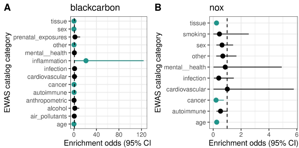
Figure 25: EWAS catalog enrichment plot: MBMS meta-analysis
