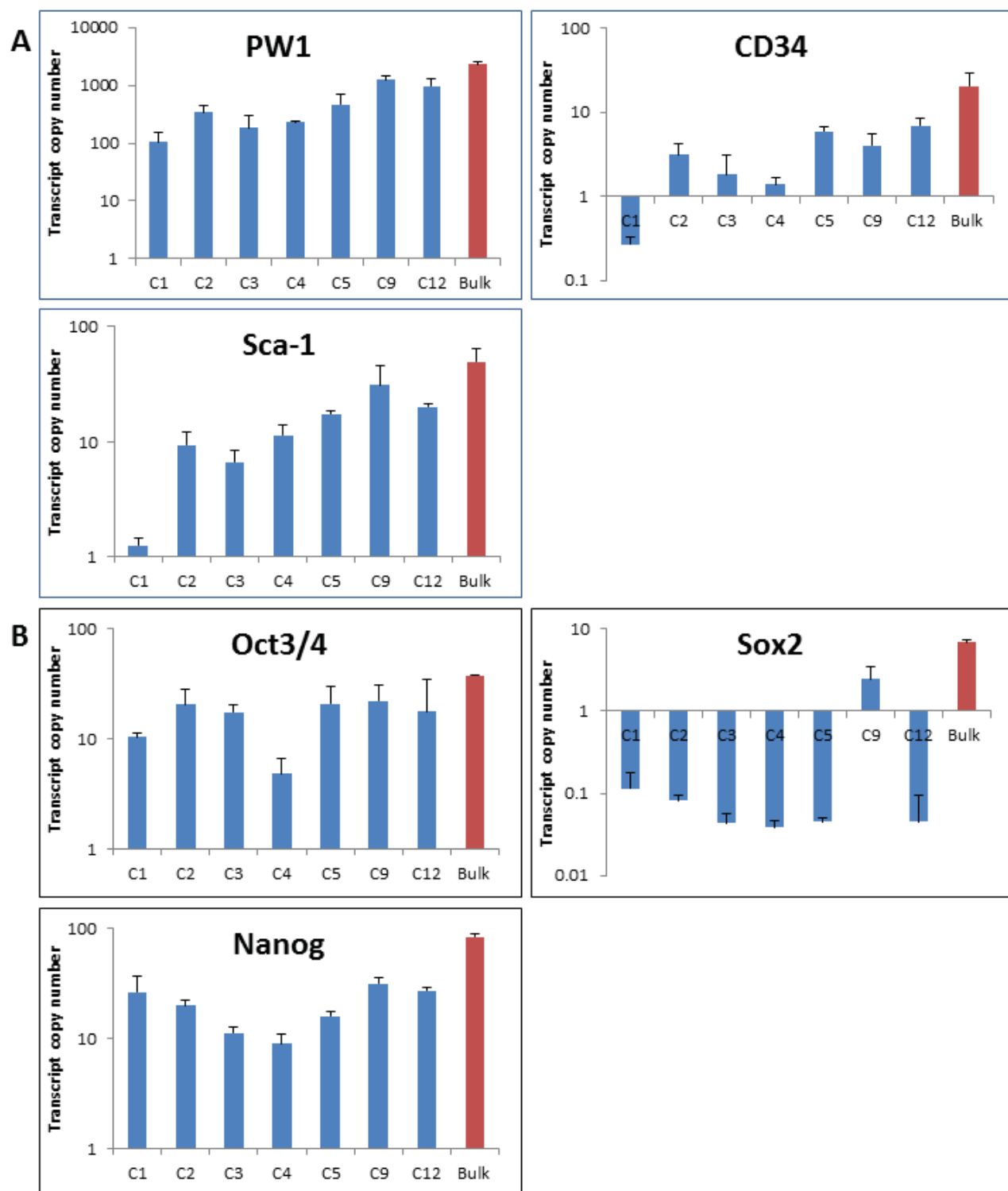
Supplementary Figure 3. Transcript analysis of clonal vs. bulk PICs. (A) qRT-PCR transcript analysis of PIC markers PW1, CD34 and Sca-1 in clonal PICs, compared to bulk PICs. (B) qRT-PCR transcript analysis of pluripotency markers Oct3/4, Sox2 and Nanog in clonal PICs compared to bulk PICs. Bars represent the mean transcript copy number normalised to GAPDH. Error bars represent the standard deviation of the mean, n=3.
