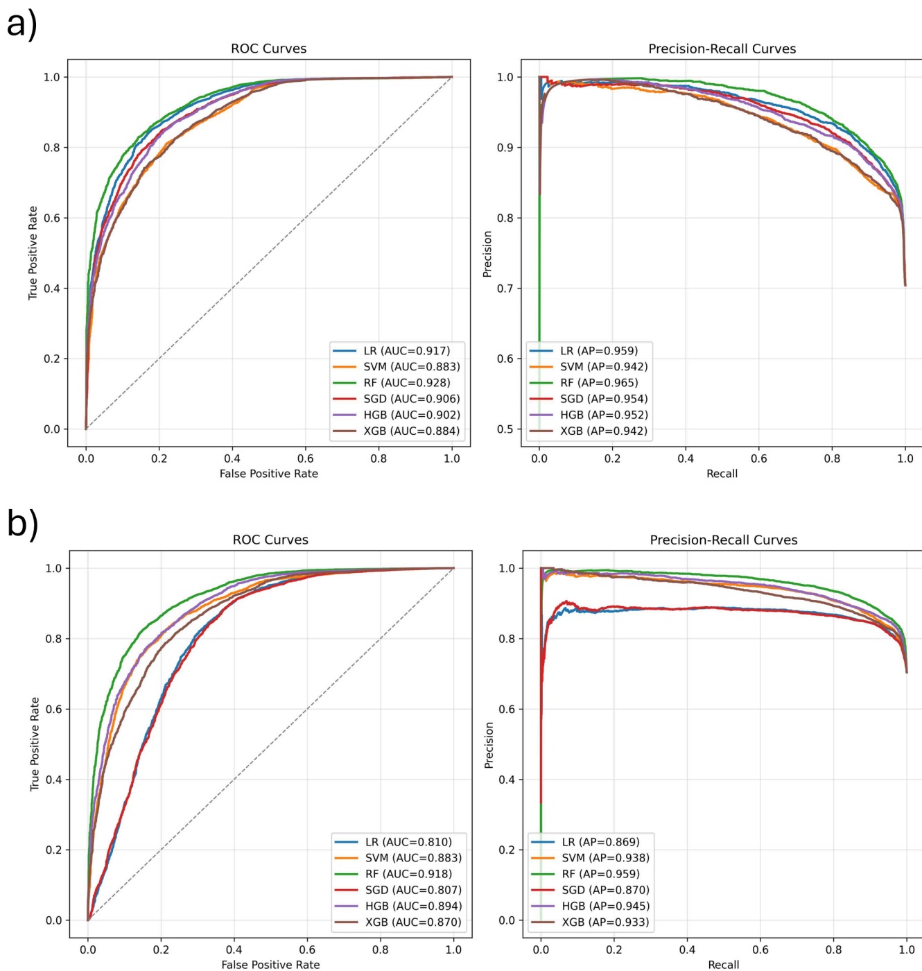
Figure S1: Receiver operating characteristic (ROC) curves (left) and precision-recall (PR) curves (right) comparing the performance of six classification models: logistic regression (LR), support vector machine (SVM), random forest (RF), stochastic gradient descent (SGD), histogram-based gradient boosting (HGB), and XGBoost (XGB) when 2.048 ECFP4 (a) and 15 theoretical features (b) have been used for training.
