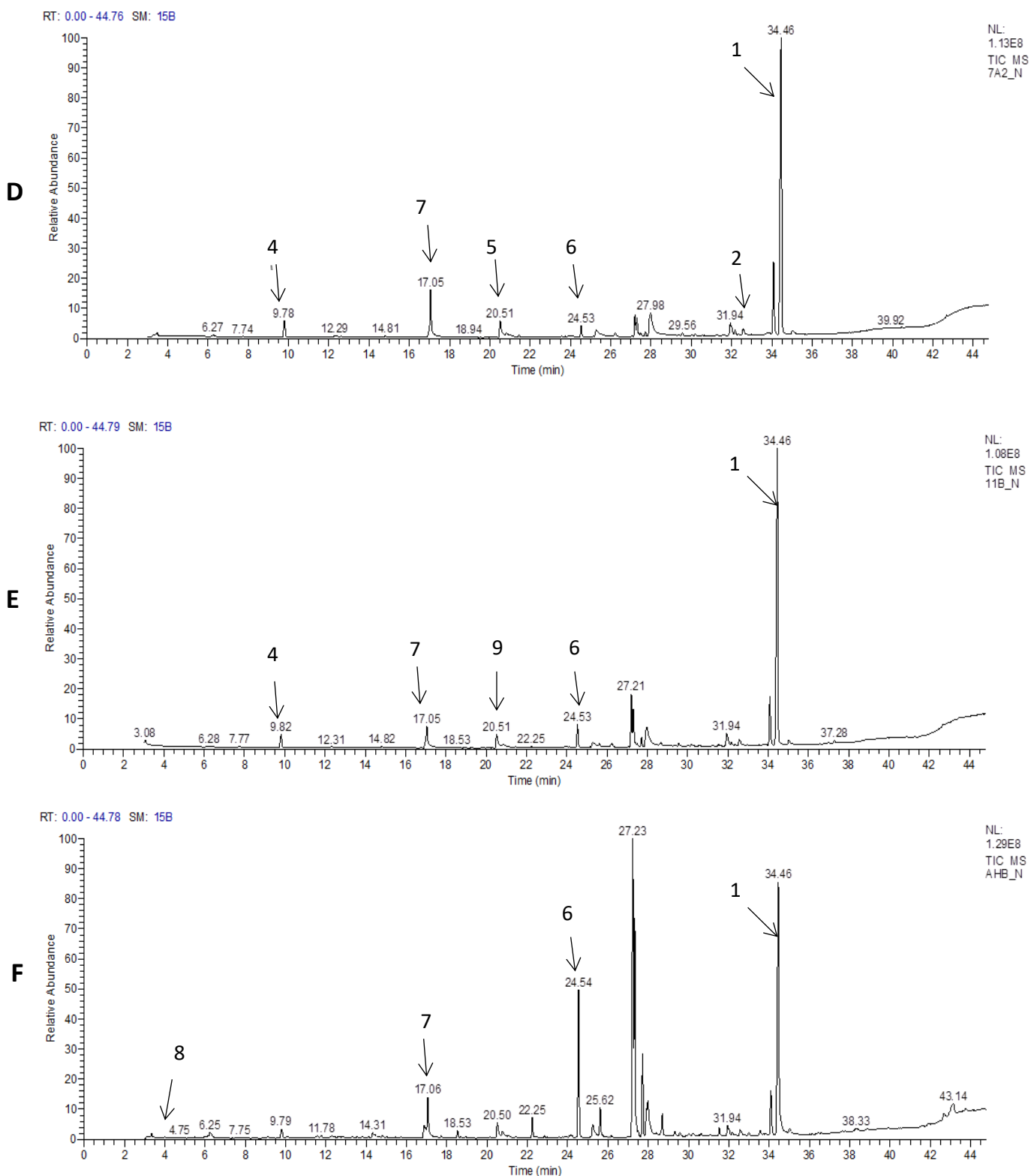
Figure S1. GC/MS profiles of MM supplemented with \lambda -Cyhalothrin after incubation for 24 h at 150 rpm and 37°C. A) GC/MS spectrum of control (non-inoculated MM+100mg/L \lambda -Cyhalothrin). B) GC/MS spectrum of MM+100mg/L \lambda -Cyhalothrin inoculated with 4B. C) GC/MS spectrum of MM+100mg/L \lambda -Cyhalothrin inoculated with 5A. D) GC/MS spectrum of MM+100mg/L \lambda -Cyhalothrin inoculated with 7A. E) GC/MS spectrum of MM+100mg/L \lambda -Cyhalothrin inoculated with 11B. F) GC/MS spectrum of MM+100mg/L \lambda -Cyhalothrin inoculated with AHB. The numbers refer to the compounds in table2.
