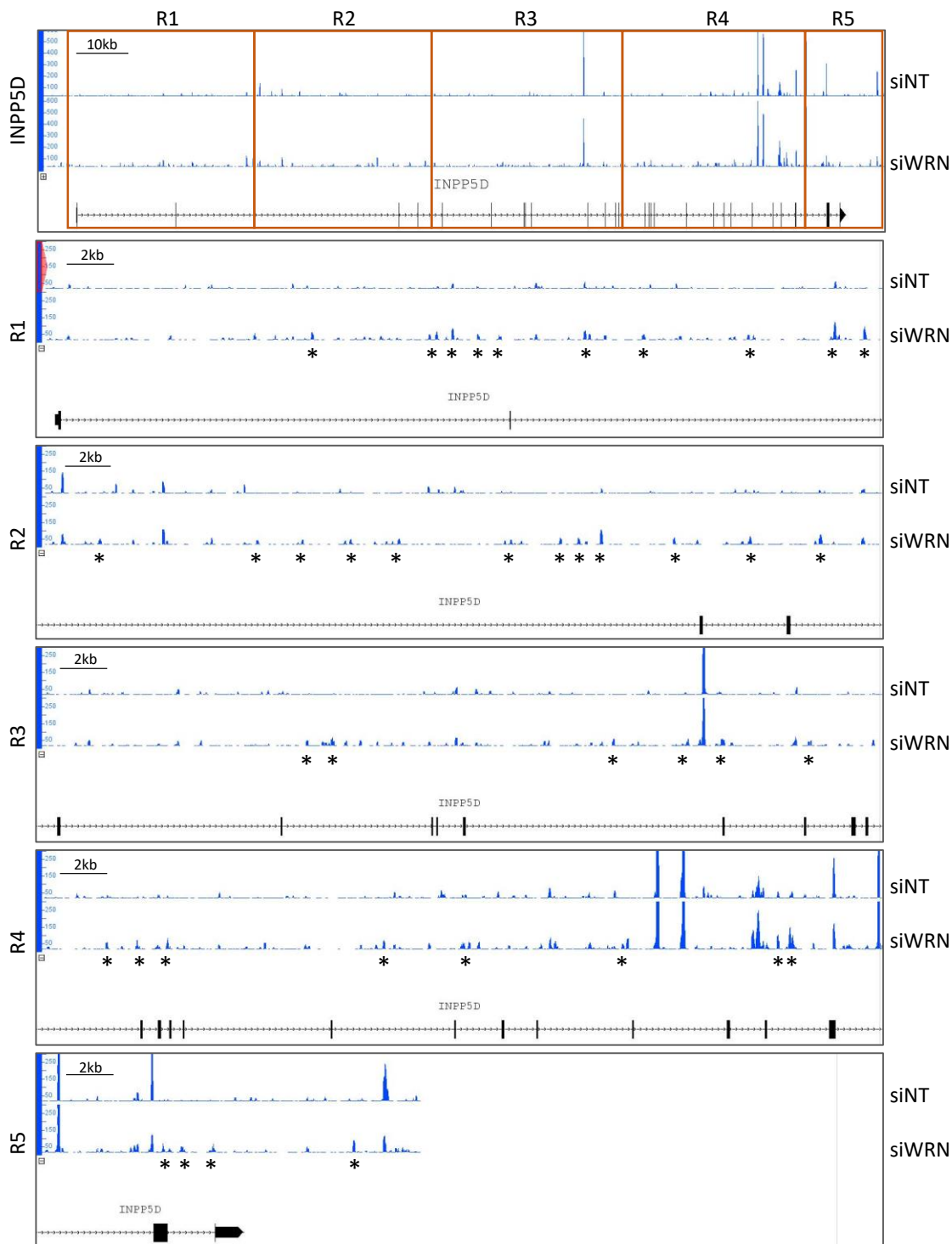
Supplementary Figure 3. G4access profiling in WRN-depleted HeLa cells (siWRN). Unprocessed data were retrieved from GEO (GSE187007) and displayed in IGB. Genomic region at INPP5D (SHIP1) was shown. Genomic regions with increased G4 peaks were highlighted with asterisks.
