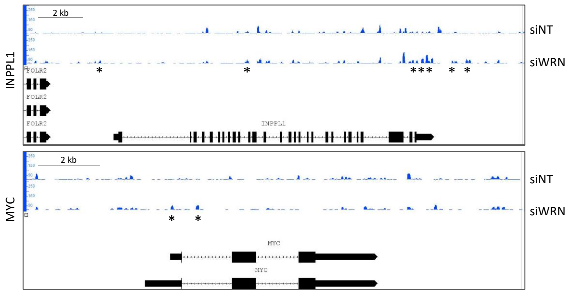
Supplementary Figure 4. G4access profiling in WRN-depleted Hela cells (siWRN). Unprocessed data were retrieved from GEO (GSE187007) and displayed in IGB. Genomic regions at INPPL1 (SHIP2) and MYC were shown. The MYC promoter contains a G4 sequence that is known target of WRN. Genomic regions with increased G4 peaks were highlighted with asterisks.
