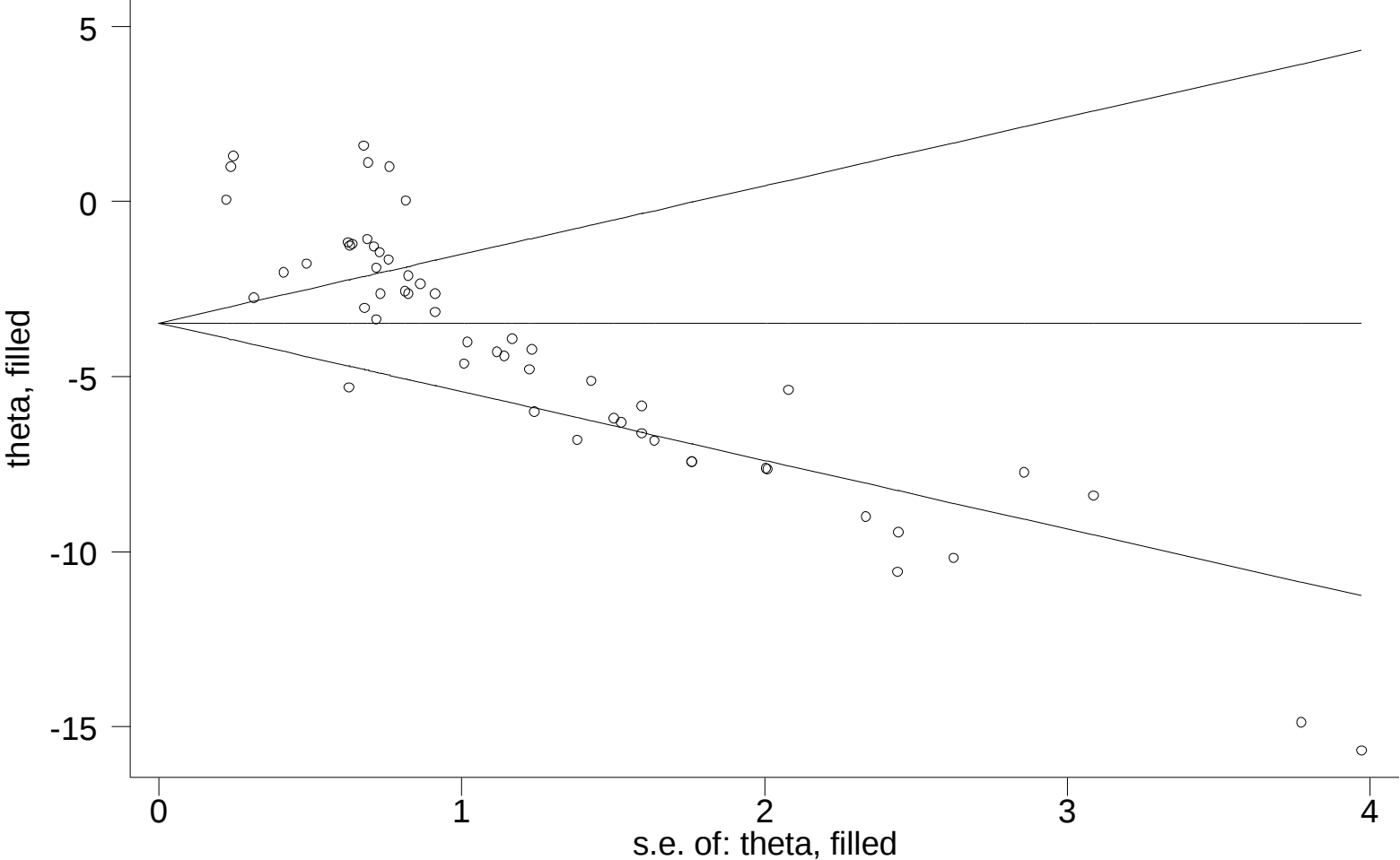
Filled funnel plot with pseudo 95% confidence limits
