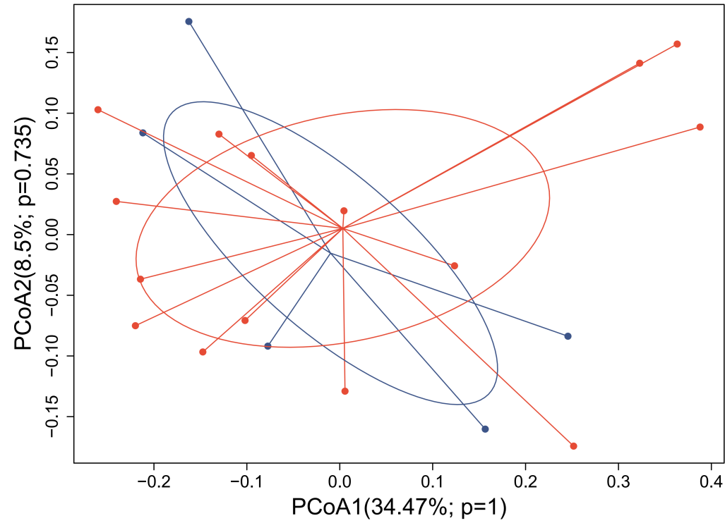
Unweighted Unifrac
