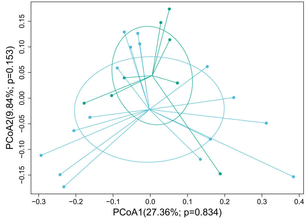
Unweighted Unifrac
