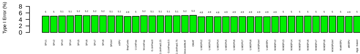
D. Logistic model: Correlated X_2
