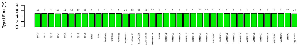
B. Linear model: Correlated X_2
