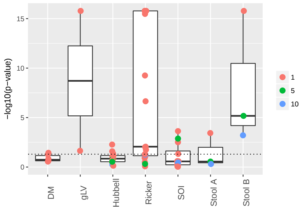
a) Neutrality test (last 100 time points)
