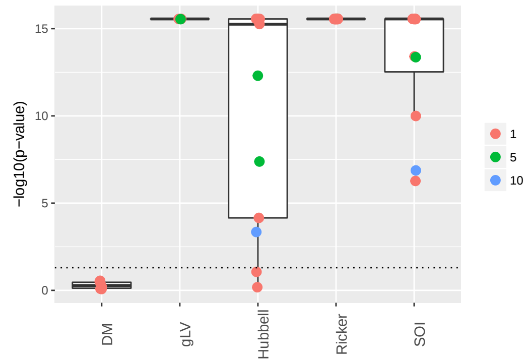
b) Neutrality test Poisson
