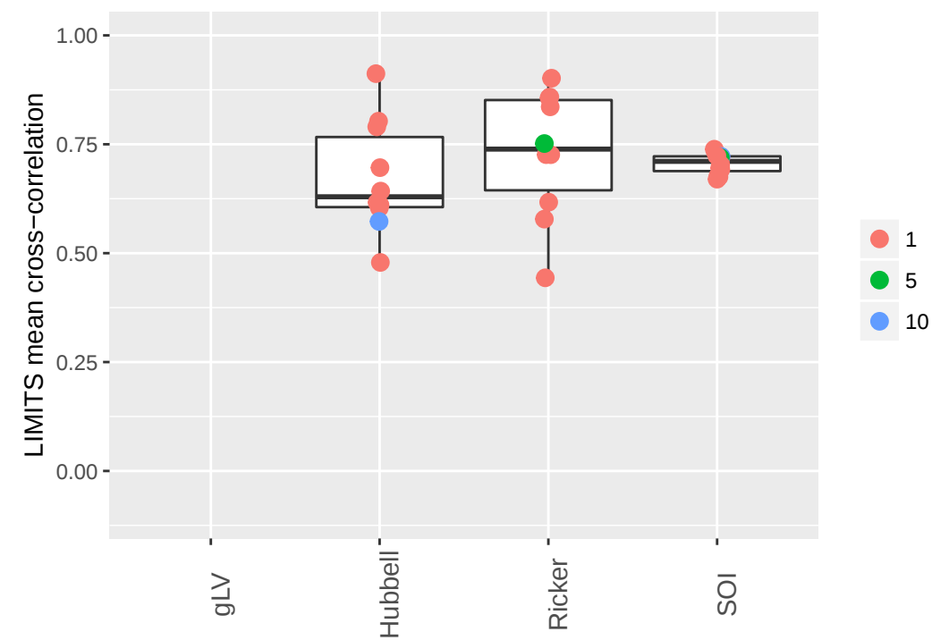
d) LIMITS goodness of fit Poisson
