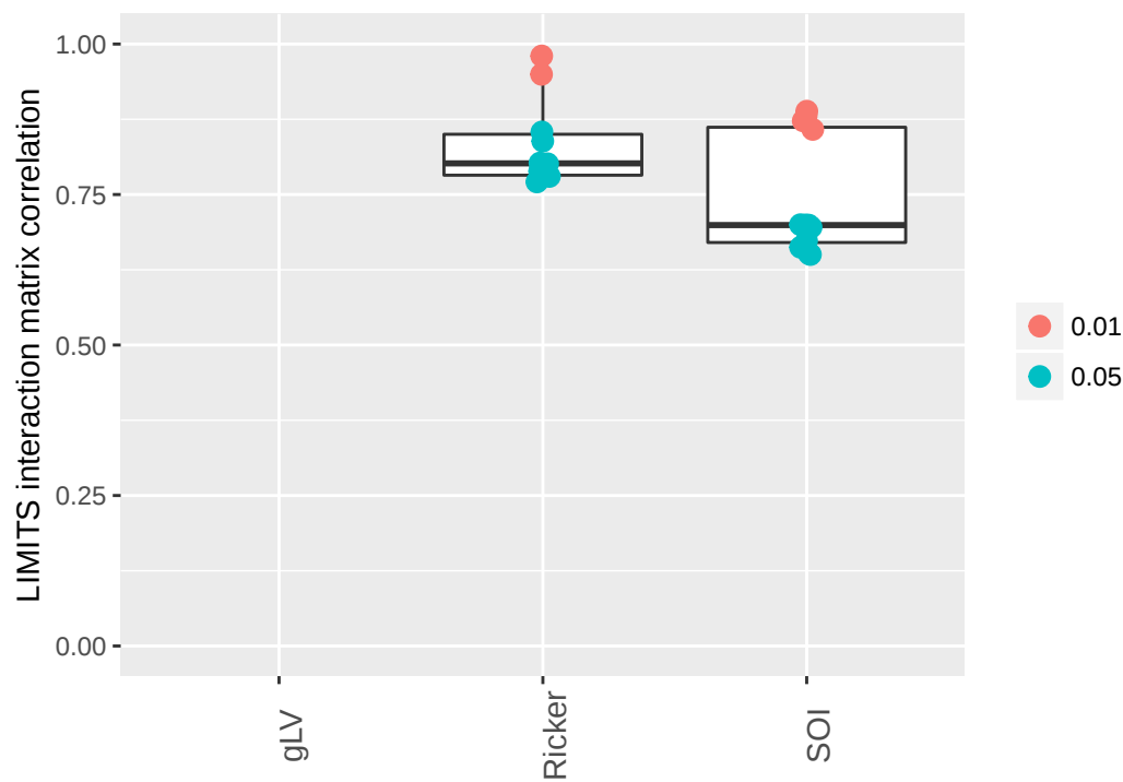
c) LIMITS accuracy Poisson
