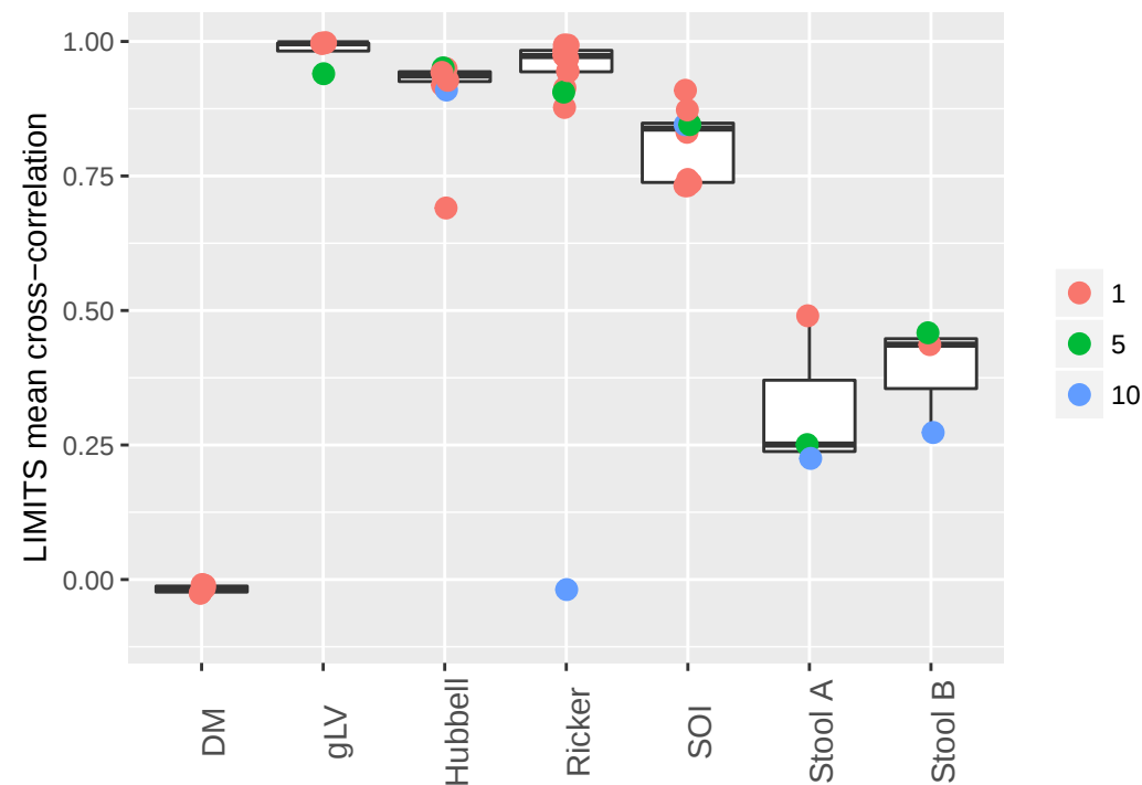
b) LIMITS goodness of fit (first 100 time points)
