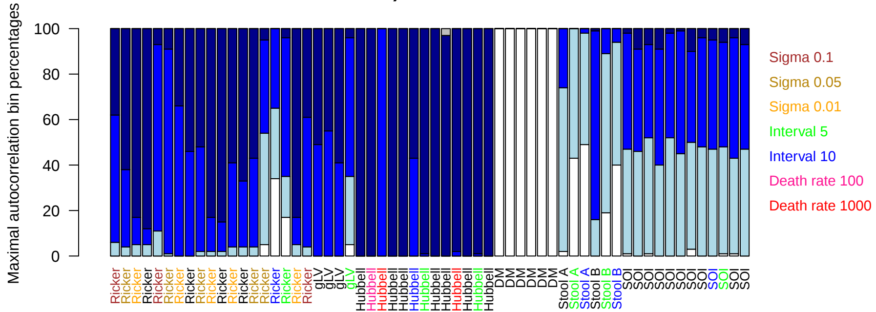
a) Maximum auto-correlation
