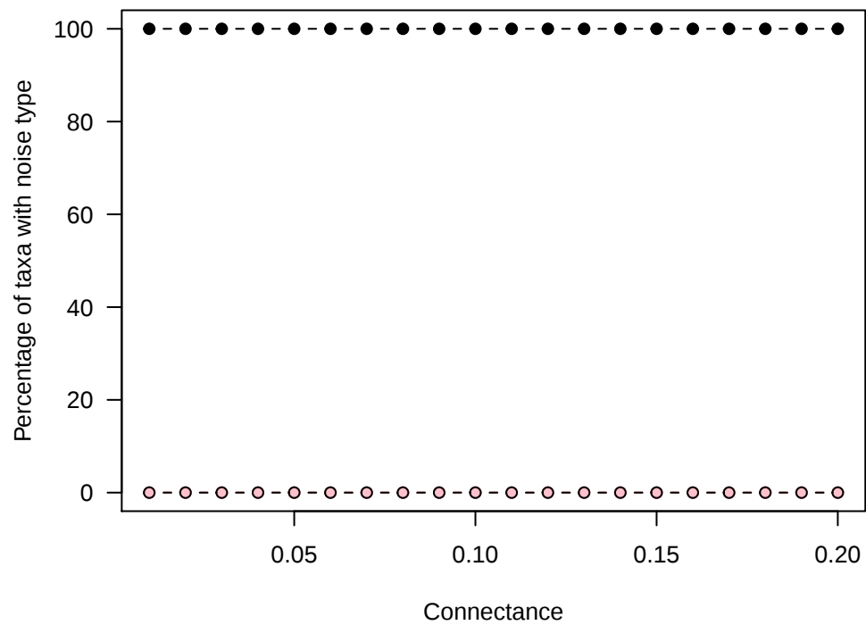
c) gLV model, PEP=20
