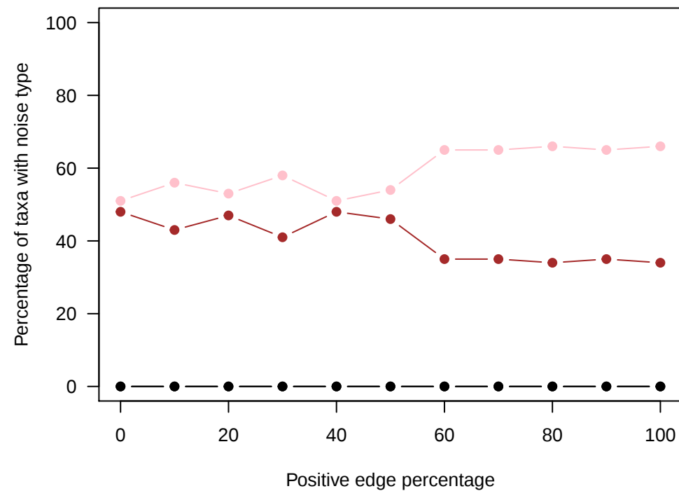
d) gLV model, c=0.01
