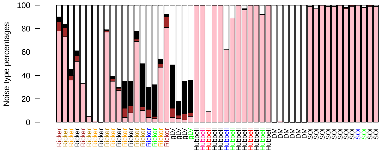
b) Noise types Multinomial
