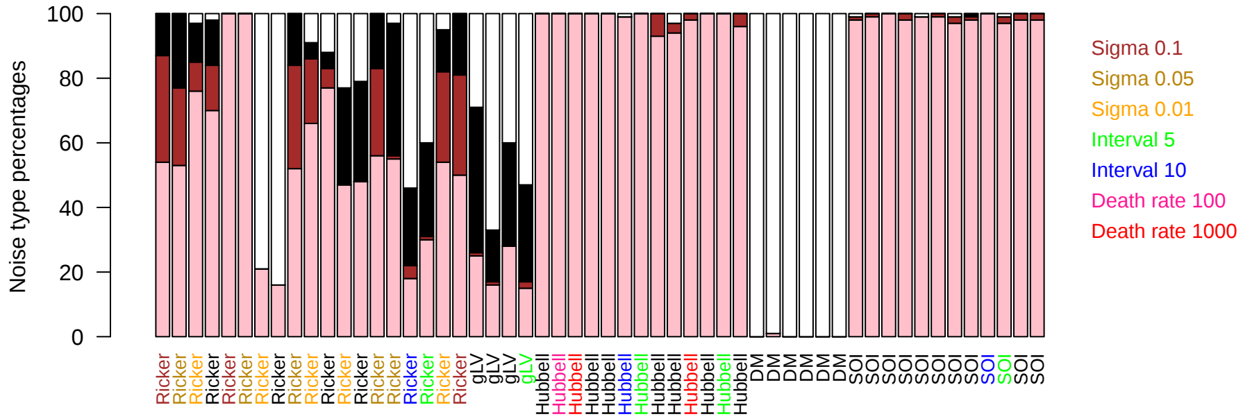
a) Noise types Poisson
