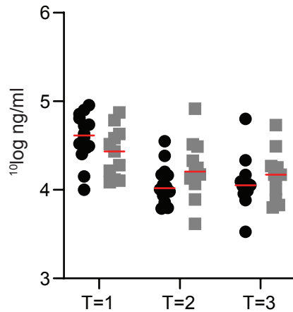
Unbound IgG
