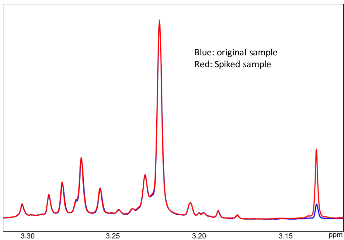
Figure S3A: 1D ^1\text{H} -NMR spectrum of a malonate spiked sample
