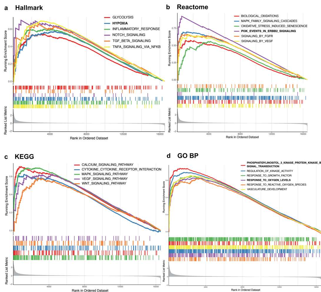
Figure S8 Functional enrichment for high HRTDGS group. (a-d) Gene sets enrichment in high HRTDGS group. The background gene sets are downloaded from Hallmark (a) , Reactome (b) , KEGG (c) , and GO BP (d) in MSigDB.
