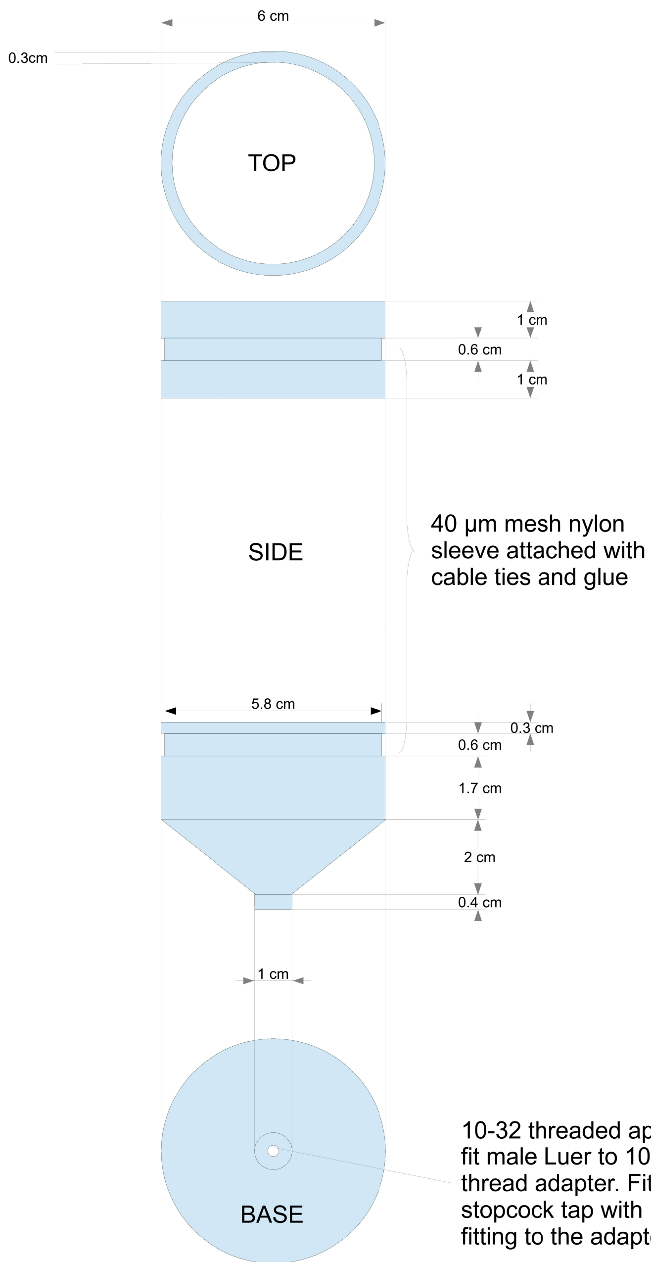
Outer funnel
