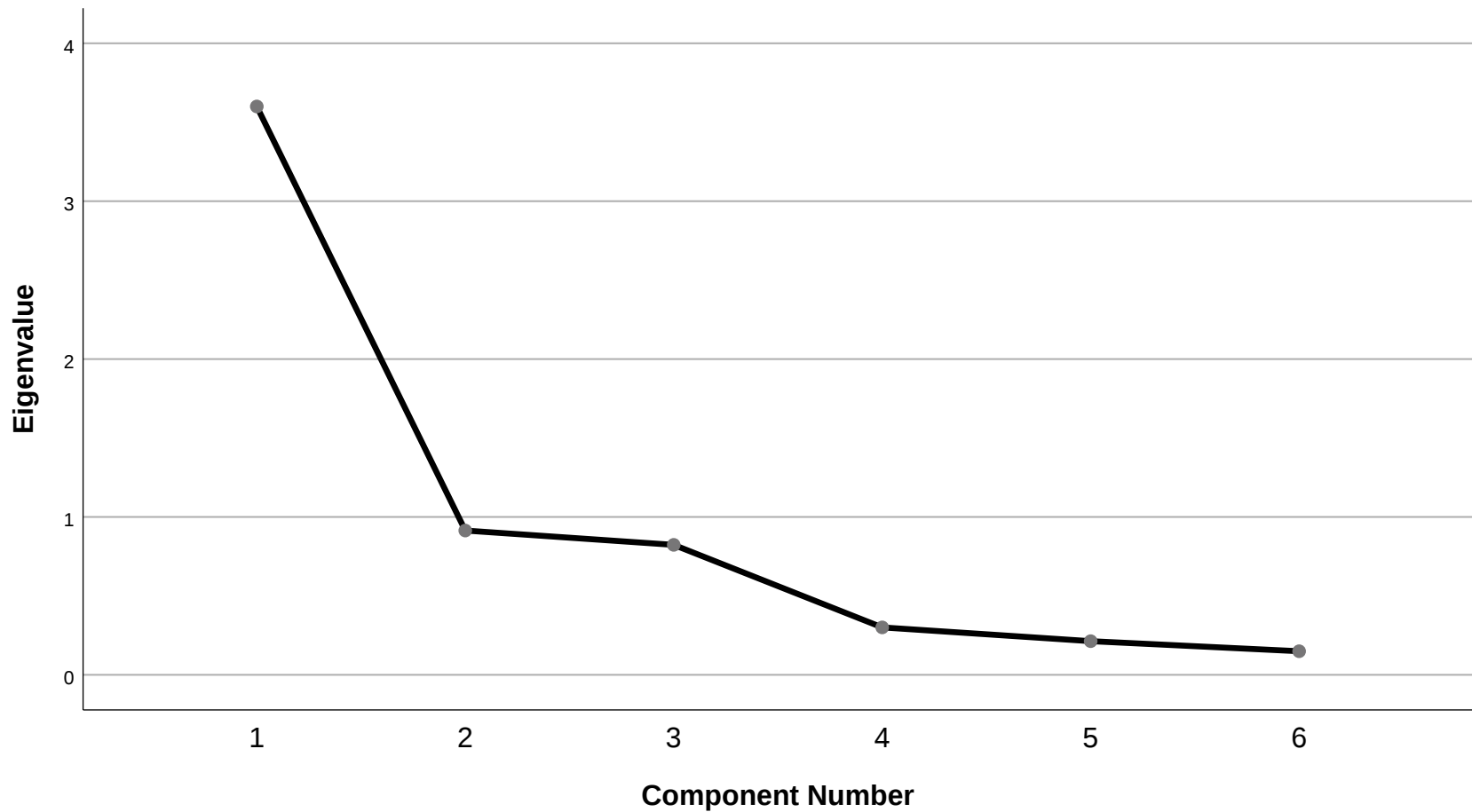
Scree Plot
