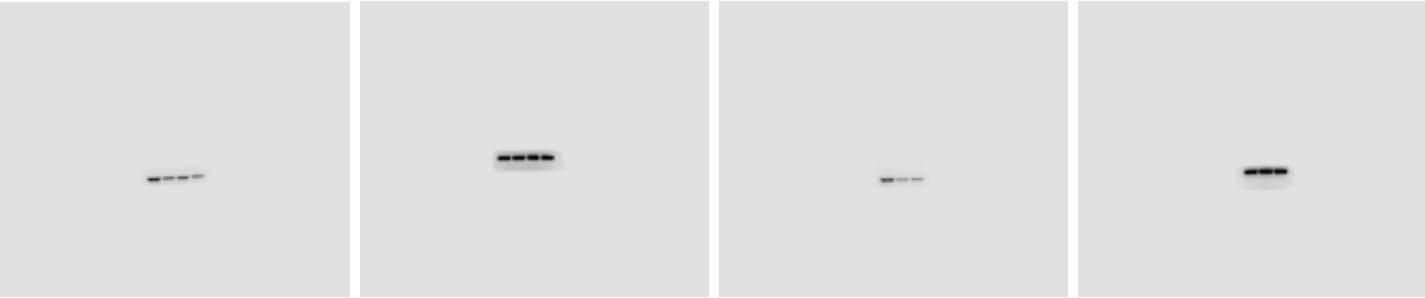
Fig. 4A blots of A549 and H1299 (The fourth lane on the right side of the A549 image is siVIM-3. We have reserved siVIM-1 and siVIM-2 as needed)
