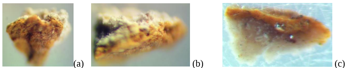
Fig. 1 Yellow sample from the Marian figure before embedding in resin for cross-sectioned preparation. Top view (a), side view (b) and cross-section preparation (c). Orpiment is identified by pXRF during on-site analysis and MRS from the cross-section shown in (c). SEM-EDS also gave similarly supportive complementary information.
