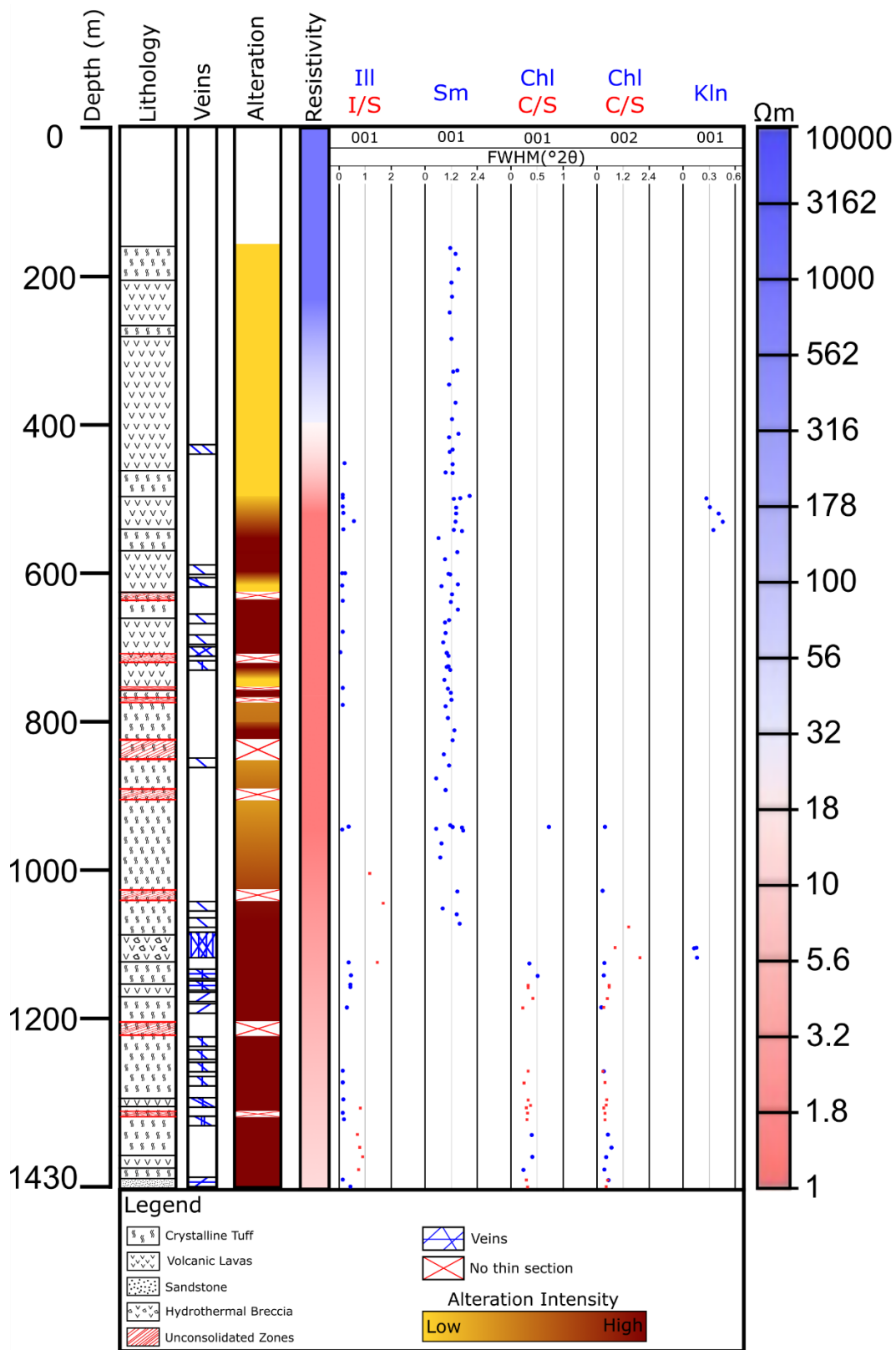
Figure 1S: Measured variations of different clay minerals crystallinities down well PGC-02. Lithology, veins, alteration intensity and resistivity are incorporated to highlight their potential effects on crystallinity. Blue dots reflect discrete clays and red dots their respective interstratification with smectite.
