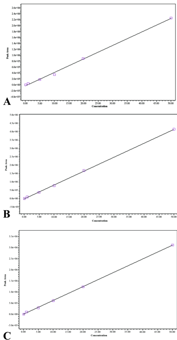
Figure S 1 Standard curves of protocatechuic acid, p-hydroxybenzoic acid, and p-hydroxyacetophenone.
