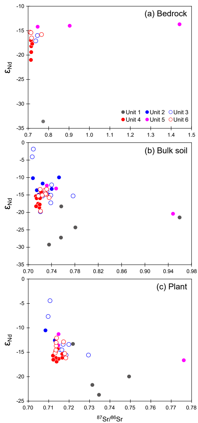
Fig. S5. The Nd versus Sr isotope plots for bedrock (a), bulk soil (b), and plant (c) samples.
