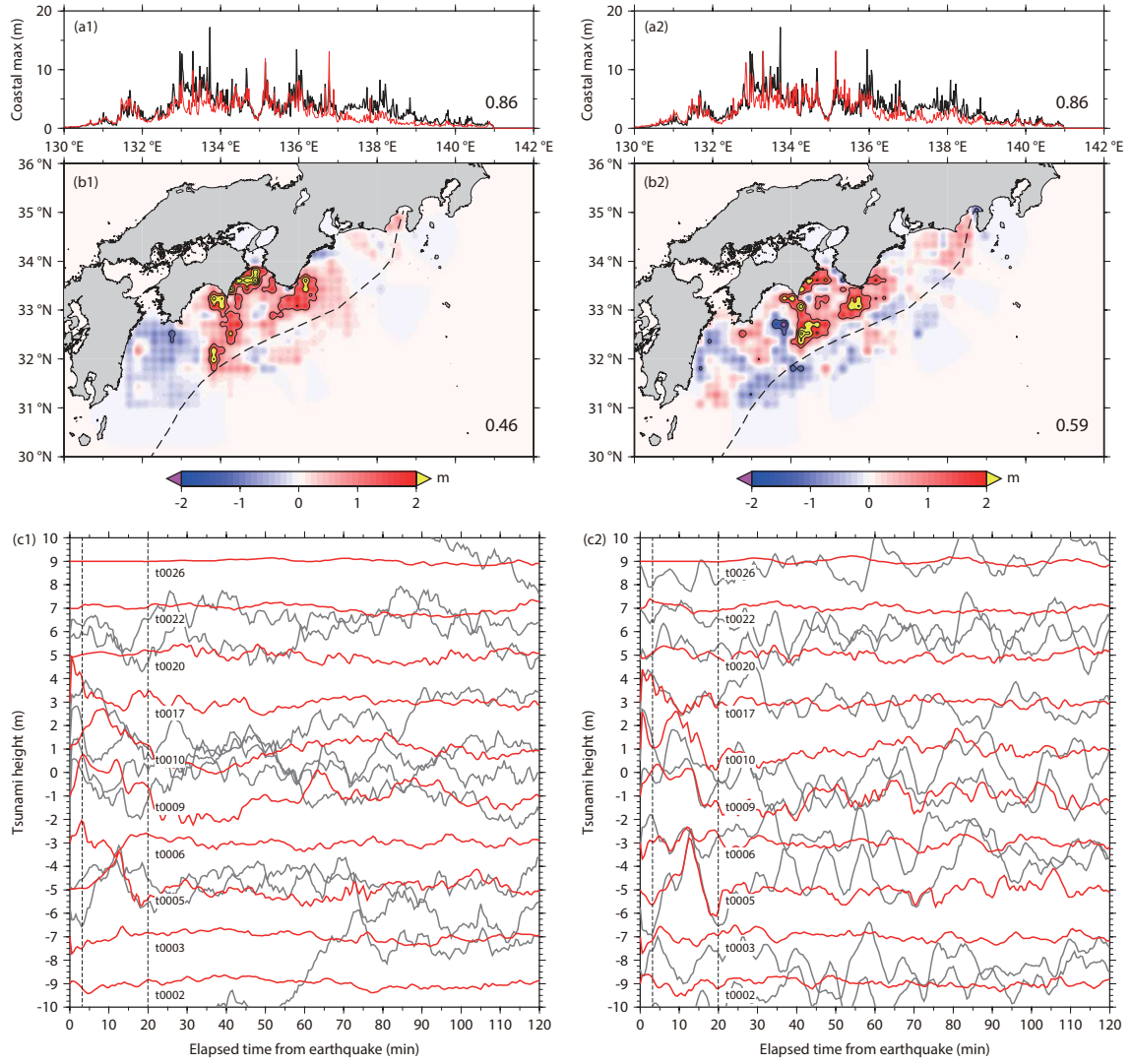
Figure S1 Forecast results. (a) Estimated maximum tsunami height (red) with that of the tsunami scenario of Fig. 2 (black). (b) Estimated tsunami source. (c) Tsunami time series at selected stations (Fig. 3b) of the estimation (red) and the pseudo observation (gray). These are the results using 3–20-min pseudo observation data from GNSS ship height (Fig. 3b). Left and right panels show the results using SINGLE ( \lambda = 1.0 ) and DGPS ( \lambda = 0.5 ) noises (Fig. 1d), respectively. Correlation coefficients between the estimation and the tsunami scenario of Fig. 2 are shown in the right-bottom sides in (a) and (b).
