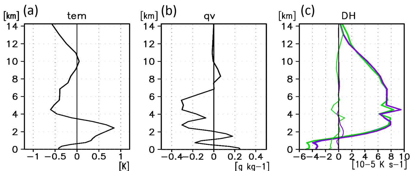
Fig. S1. Vertical profiles of (a) temperature and (b) water vapor content differences (E_mp2 minus N_mp2) averaged for the initial three hours, and (c) latent heating rate in E_mp2 (blue), E_mp4 (green), and N_mp2 (purple) averaged for the 6-day integration (the difference from E_mp2 is also plotted by thin lines), over the (120-160E, 10S-20N) domain.
