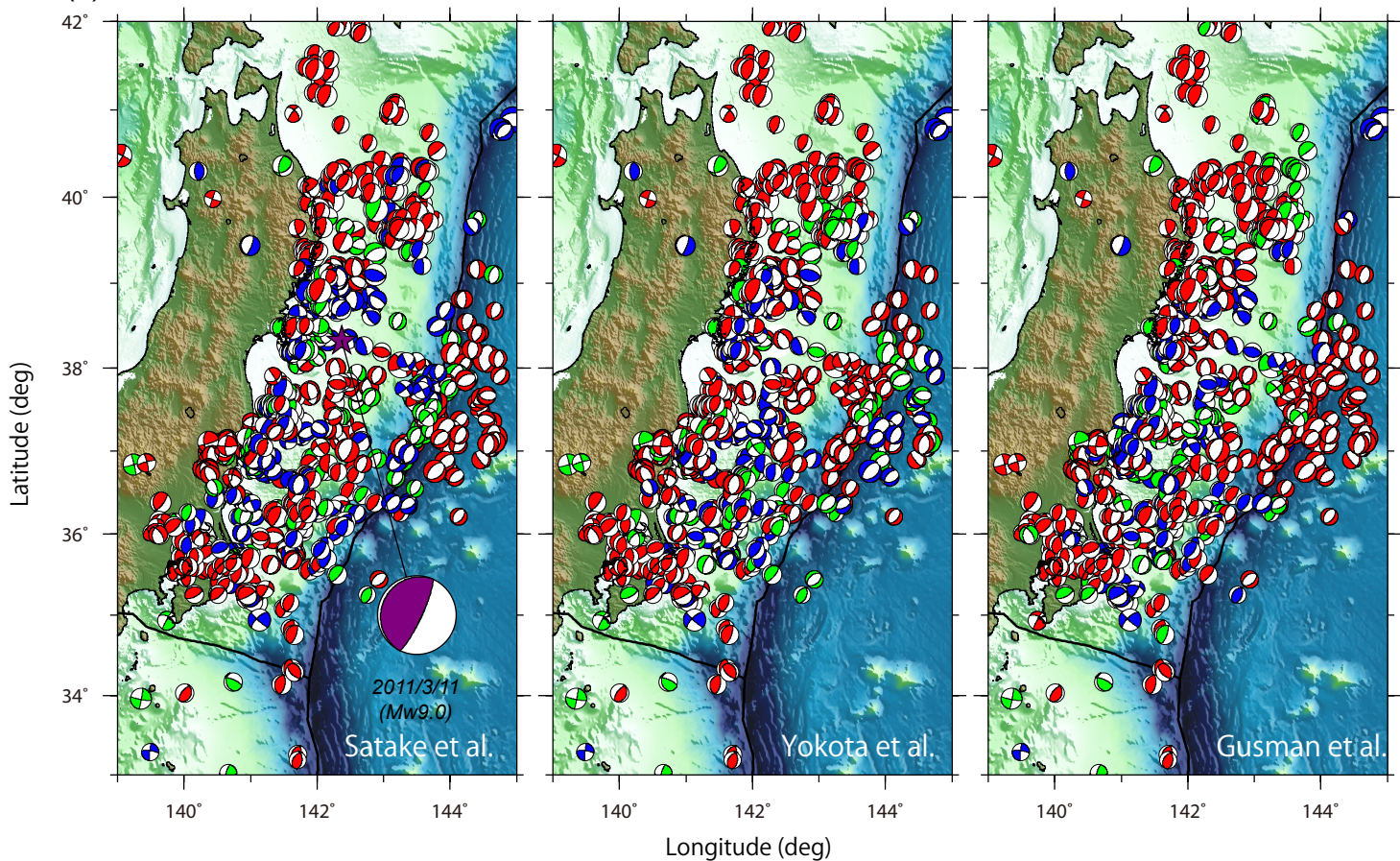
(b) Post-seismic
