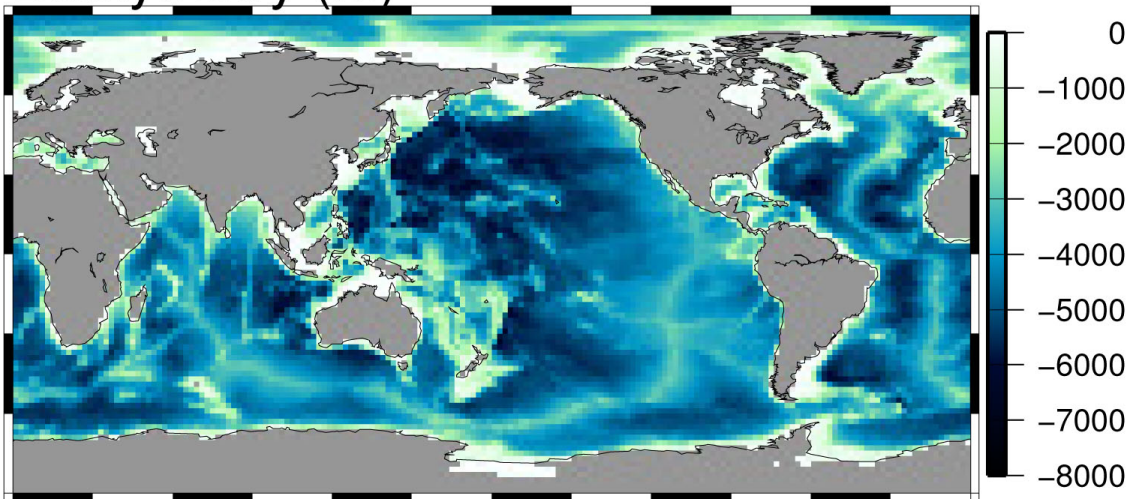
Sediment thickness (m)
