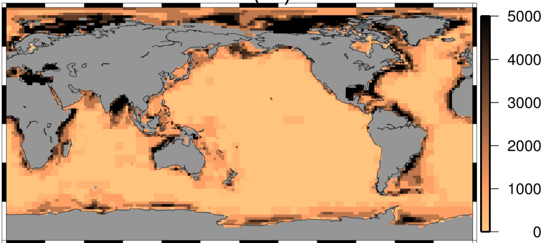
Crust thickness (km)
