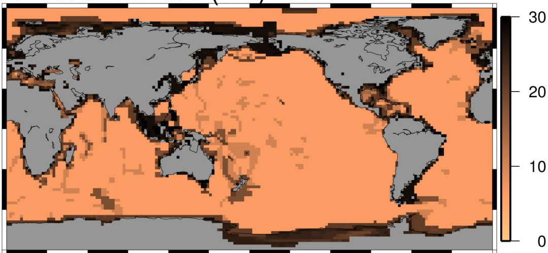
Figure A. Bathymetry, sediment thickness, and crust thickness from CRUST2.0.
