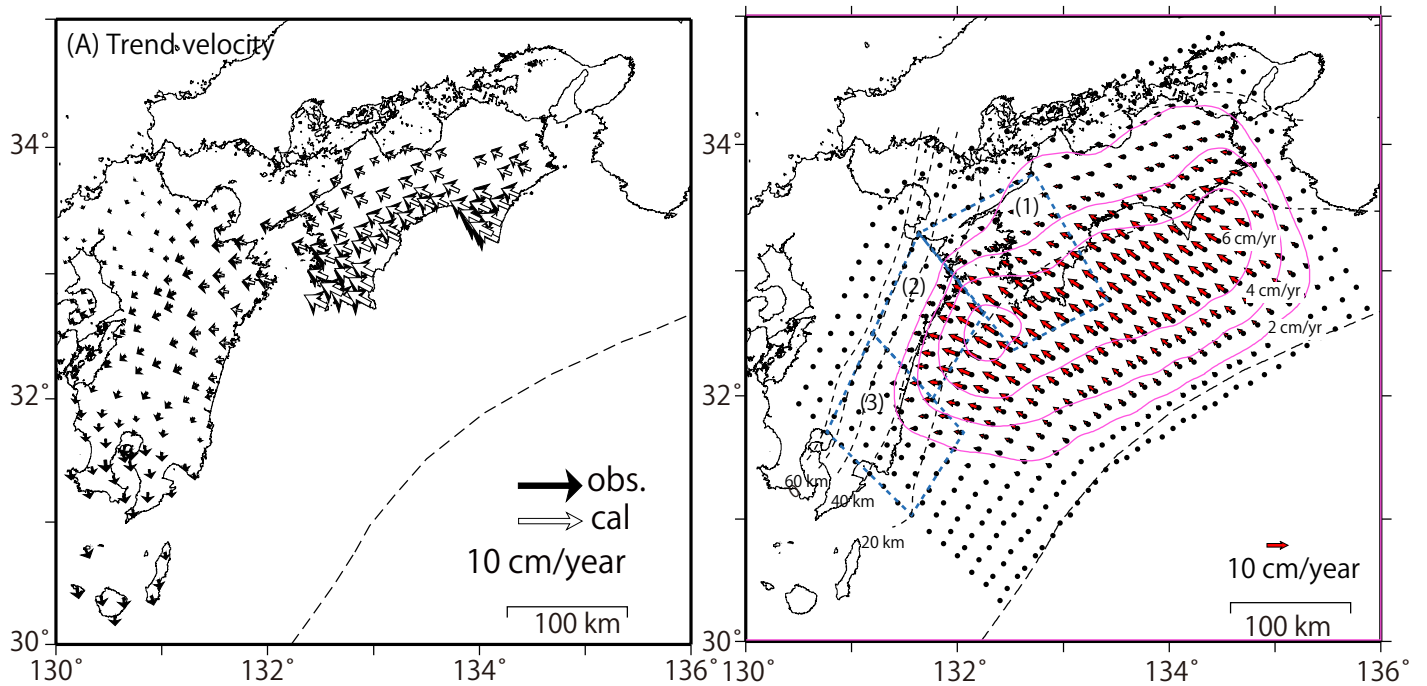
Additional file 5. (A) Trend velocity estimated for the period between January 2012 and March 2013. Black and white arrows indicate observation and computation values, respectively. (B) Slip deficit rates (red arrows) estimated by applying the method of Yabuki and Matsu'ura (1992) to the data in (A). Purple contour indicates slip magnitude with contour interval of 2 cm/year. Broken lines indicate the iso-depth contours of the upper surface of the Philippine Sea plate with a contour interval of 20 km.
