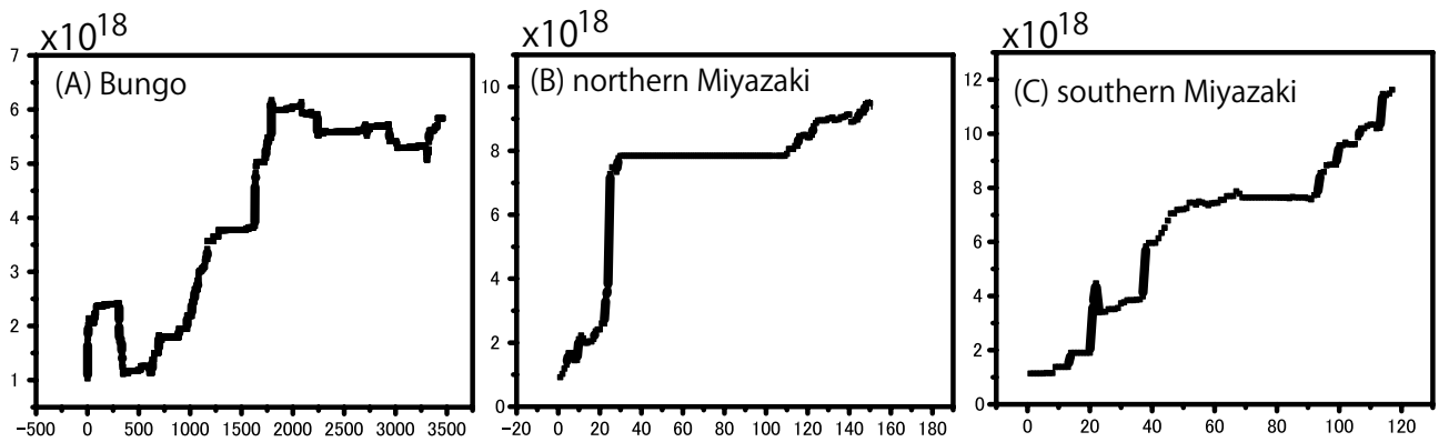
Additional file 6. Estimated aseismic moment ( \text{Nm} ) plotted against the number of earthquakes. Aseismic moments are computed on the three segments denoted by blue dashed lines shown in Fig. 4h. The number of earthquakes within 5 km from each segment is indicated. (A) corresponds to the northernmost segment in Fig. 4h. (B) corresponds to the middle segment in Fig. 4h. (C) corresponds to the southernmost segment in Fig. 4h.
