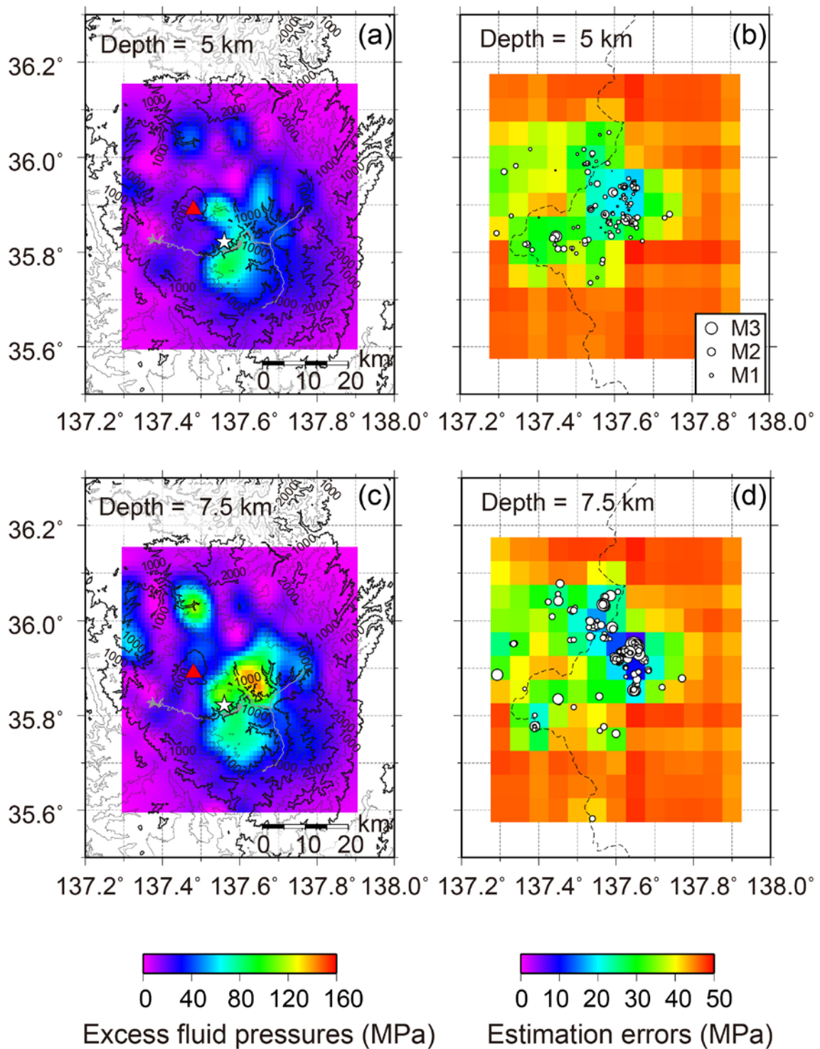
Additional file 1: The 3-D pore-fluid pressure field around Mt. Ontake estimated in Terakawa et al. (2013). (a) Pore-fluid pressures at a depth of 5 km. (b) Estimation errors of pore-fluid pressures at a death of 5 km. (c) Pore-fluid pressures at a death of 7.5 km. (d) Estimation errors of pore-fluid pressures at a death of 7.5 km. The pore-fluid pressure fields are superposed on the topographic map in (a) and (c). The white circles
