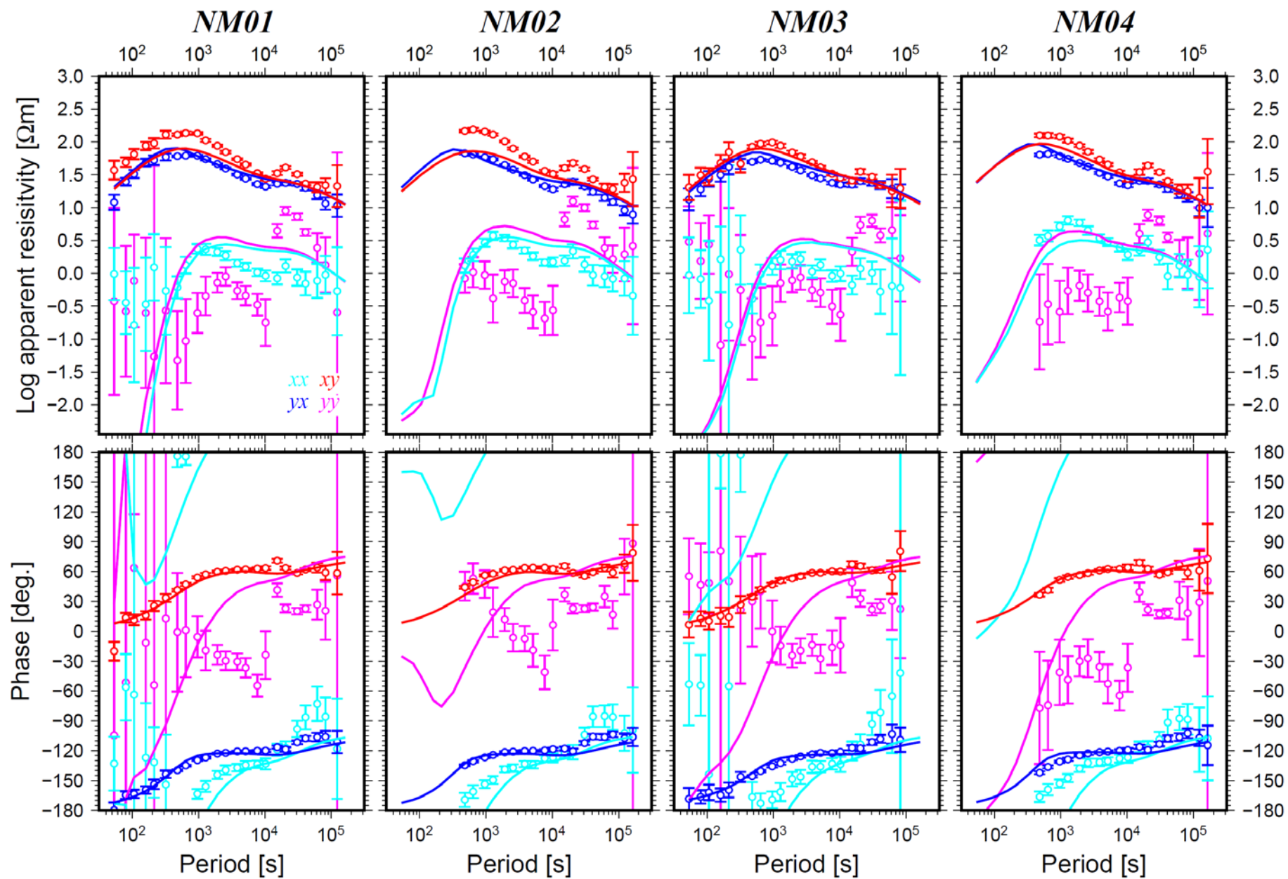
Figure S1. MT responses for all site in Area A and Area B in terms of log apparent resistivity (top) and impedance phase (bottom) sounding curves. Symbols and lines are the same as those in Figure 3.
