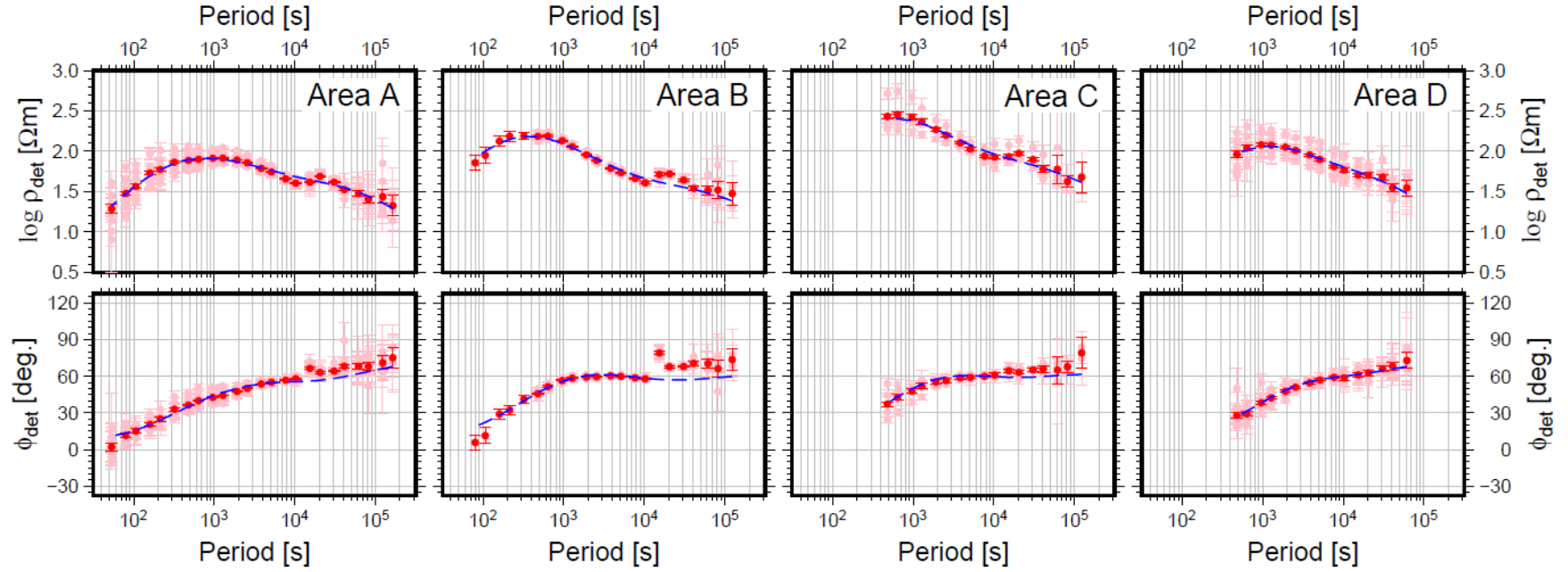
Figure S3. Apparent resistivity and impedance phase sounding curves of \bar{Z}_{\text{det}}(T) (red) and Z_{\text{det}}(\mathbf{r}, T) for each site (pink) after topographic effect correction for four areas in the northwestern Pacific (Figure 1). Error bars indicate 95% confidence limits. Blue dashed lines are the model responses calculated from the 1-D profiles shown in Figure 11.
