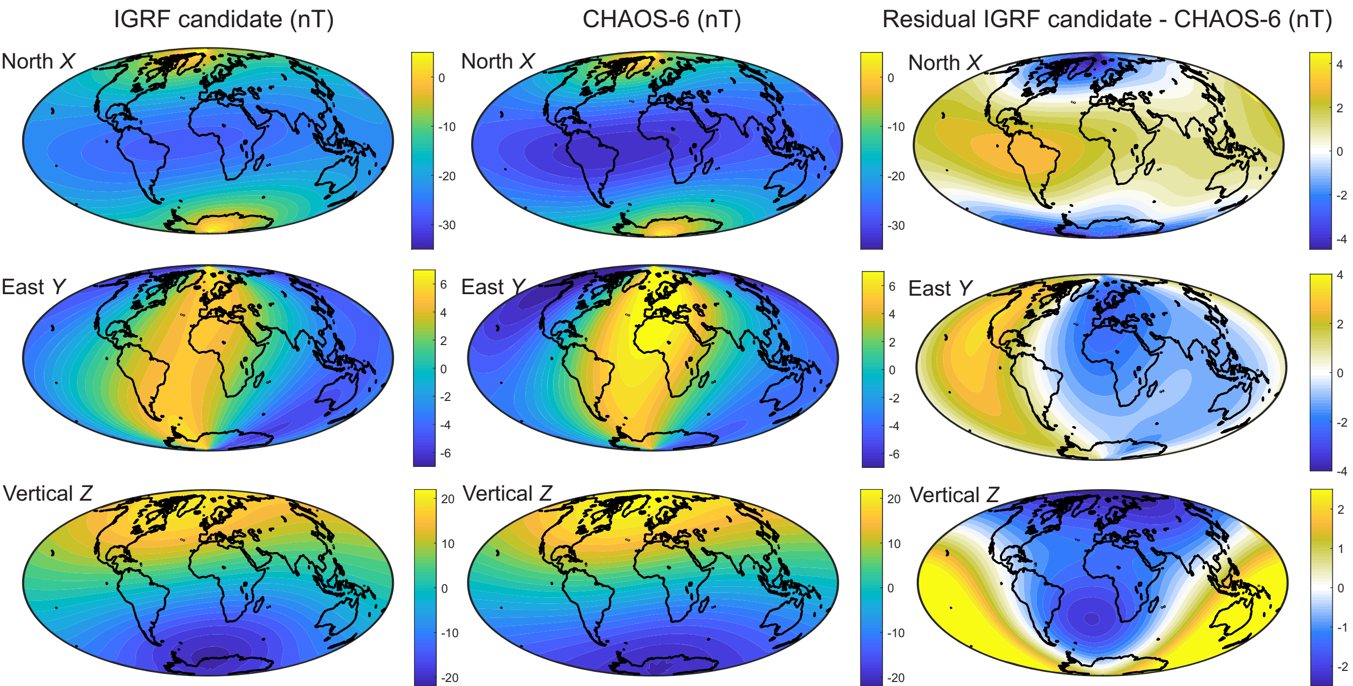
b) External field at 2019.16 from IGRF parent model and CHAOS-6 model.
