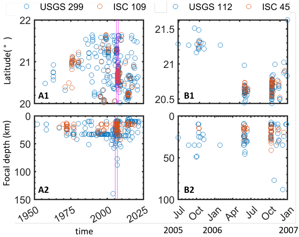
Figure S2. The temporal evolution of the seismicity illustrated by latitude (A1 and B1) and focal depth (A2 and B2) sections. (A1) and (A2): events inside the purple rectangular in Figure S1. (B1) and (B2) events in the period from July 2005 to December 2006. Two pink lines in A1 and A2 indicate the begin and end times for (B1) and (B2).
