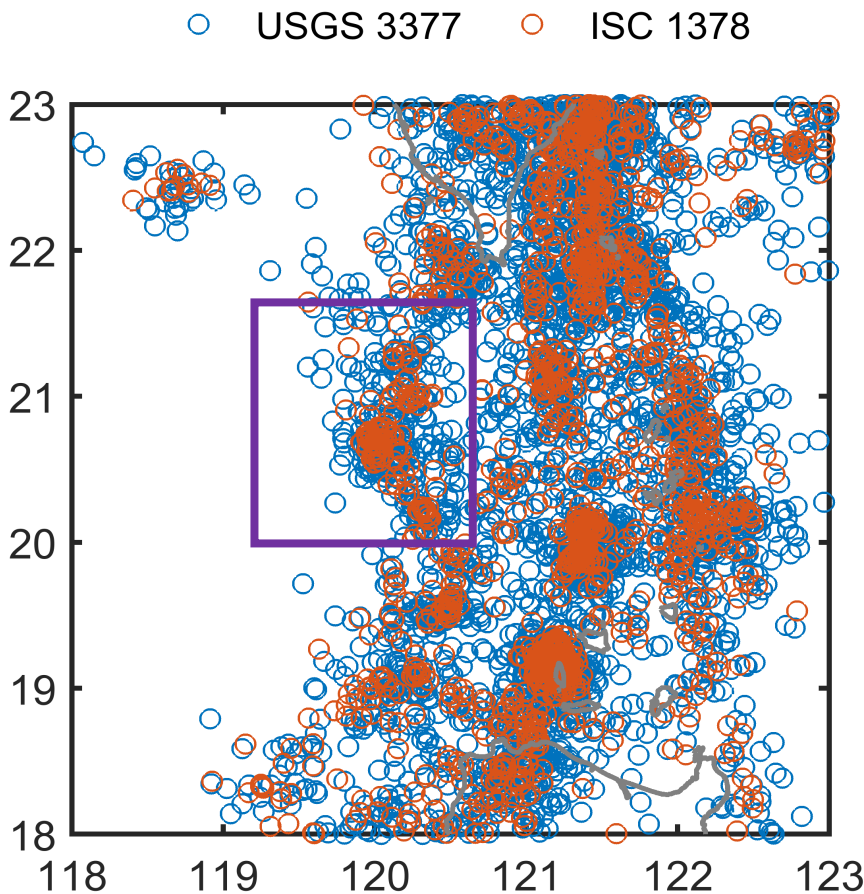
Figure S1. The epicentral distribution of the events archived in the USGS and ISC-EHB catalogs. The event numbers of each catalog are shown at the title line.
