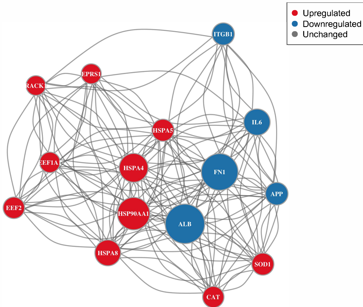
Supplemental Figure 10 Top 15 Hub Proteins: Early LVt vs Early APRV
