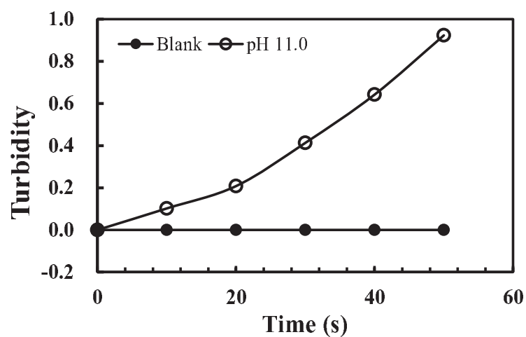
Figure S5. Initial precipitation rates of \text{CaCO}_3 catalyzed by LdCA at pH 11.0. The intrinsic turbidities of the cells were subtracted from the curves.
