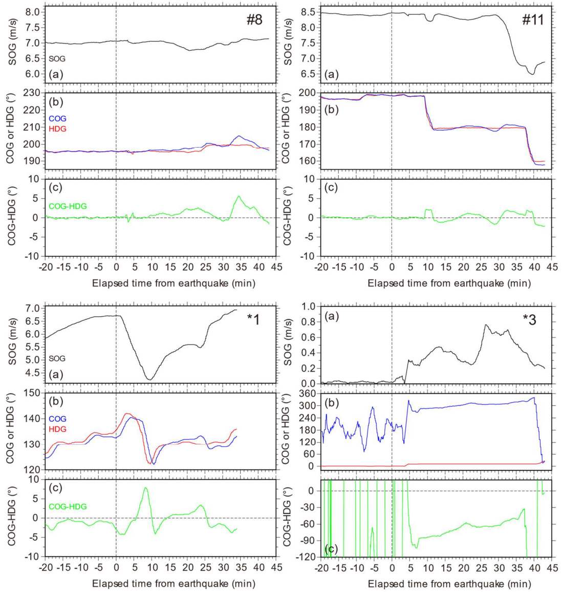
Figure S1 (a) SOG, (b) COG/HDG, and (c) COG minus HDG of selected ships (#8 and #11 for upper panels and *1 and *3 for lower panels). #8 and #11 are examples that were used for the tsunami current analysis (See also Fig. 4). *1 and *3 were not used due to the data quality issues noted in Table 1.
