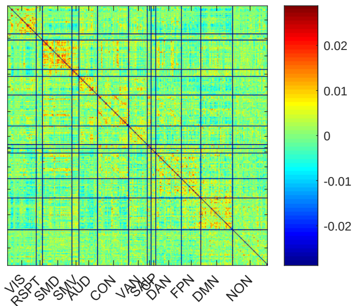
Feature 28 Weight = -0.1311
