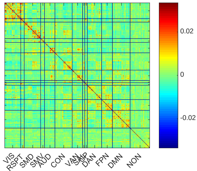
Feature 2 Weight = -0.4095
