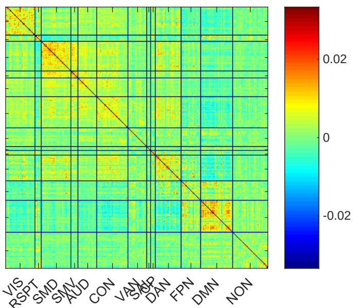
Feature 26 Weight = 0.1035
