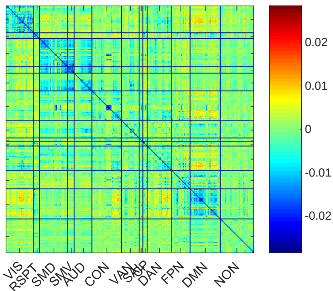
Feature 9 Weight = 0.3911
