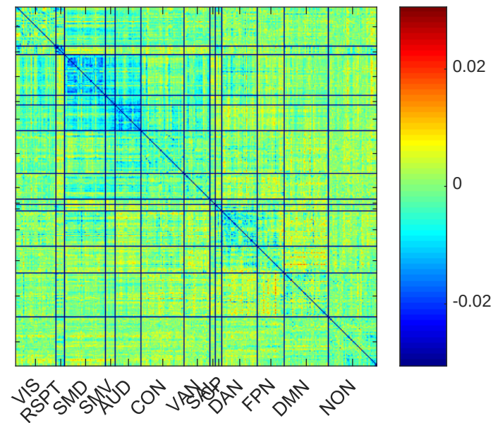
Feature 27 Weight = -0.2808
