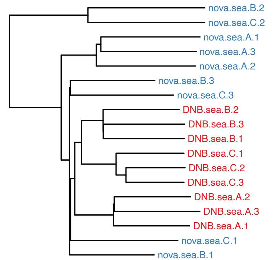
unweighted_unifrac cluster tree
