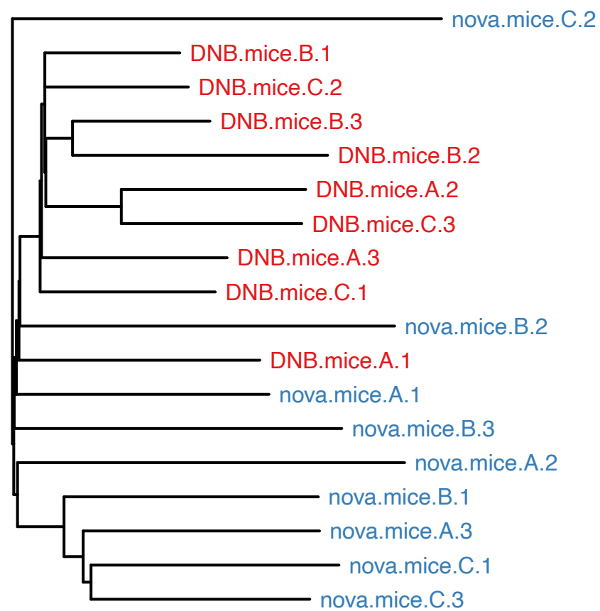
unweighted_unifrac cluster tree
