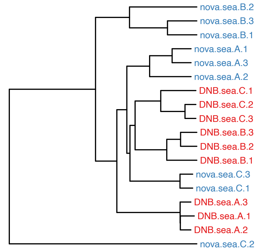
weighted_unifrac cluster tree
