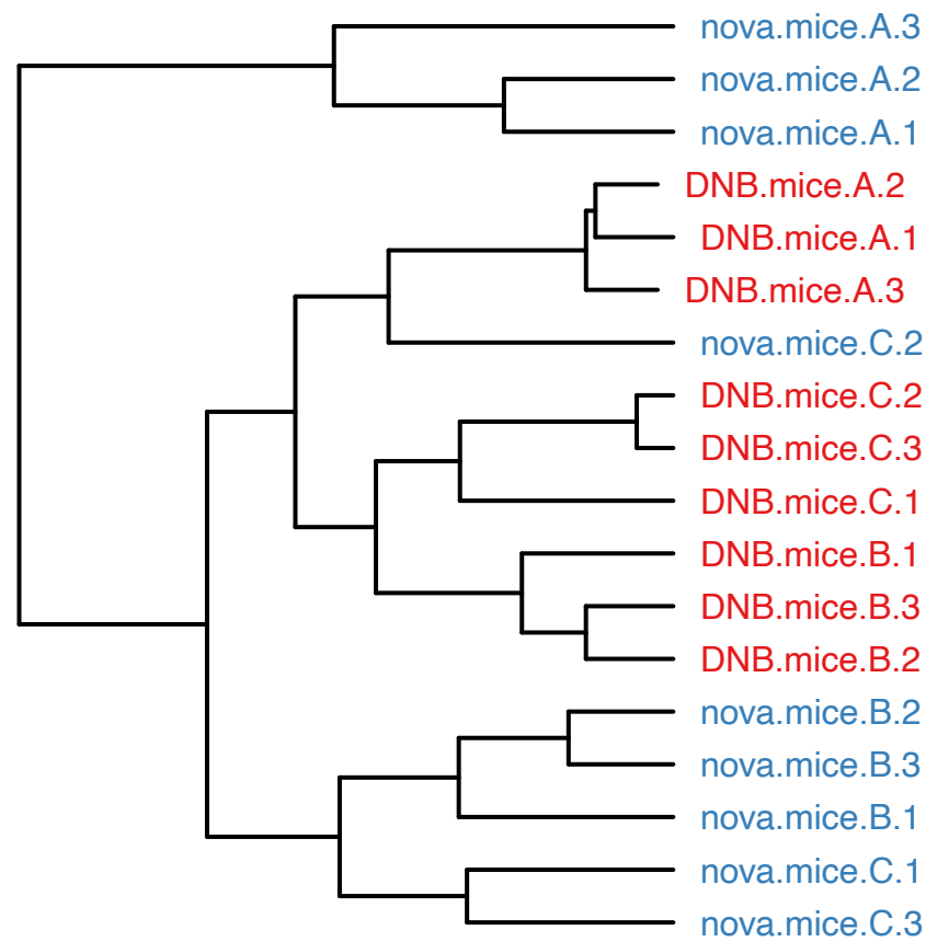
weighted_unifrac cluster tree
