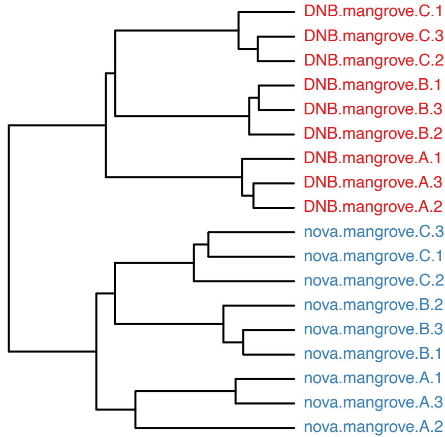
weighted_unifrac cluster tree
