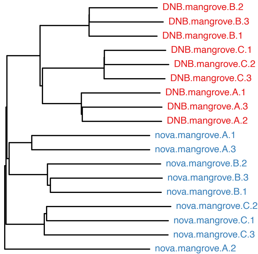
unweighted_unifrac cluster tree
