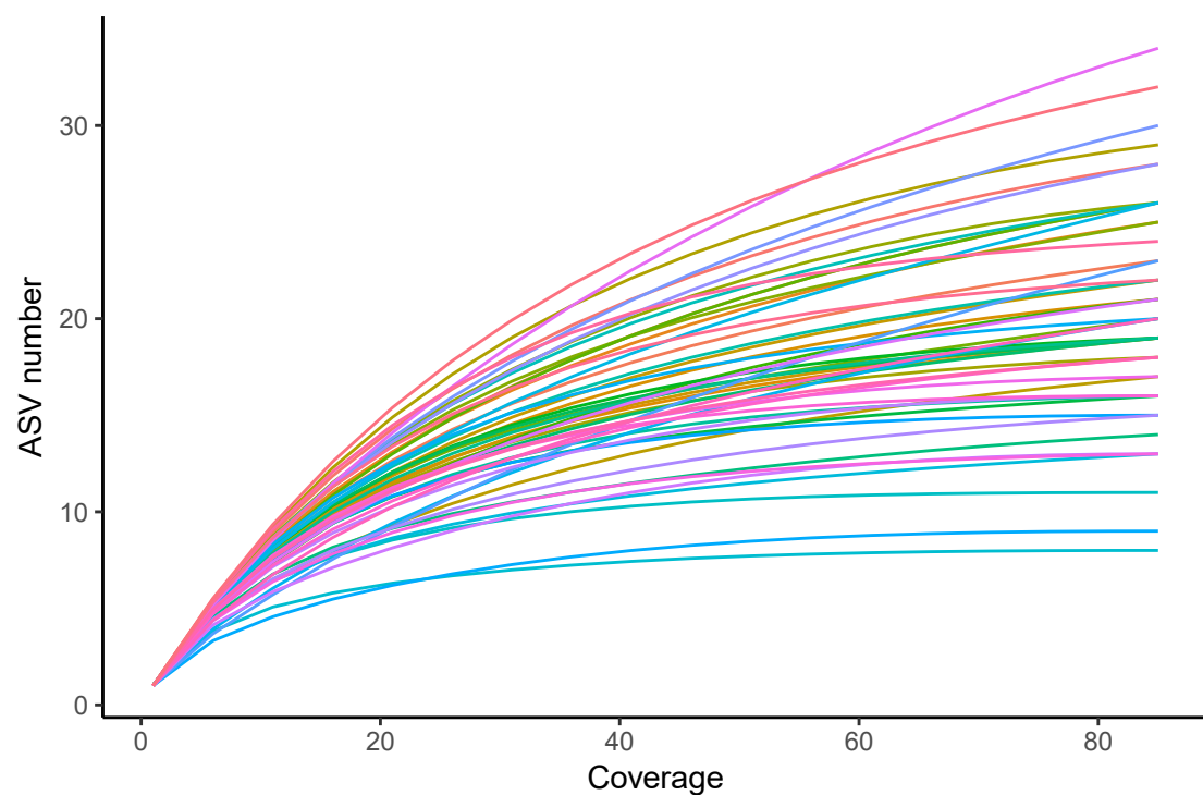
Rarefaction curve normalized seed samples
