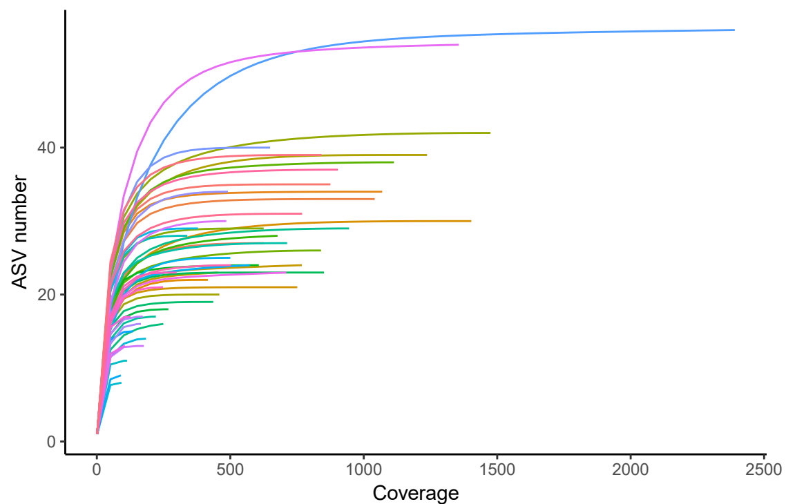
Rarefaction curve non-normalized seed samples
