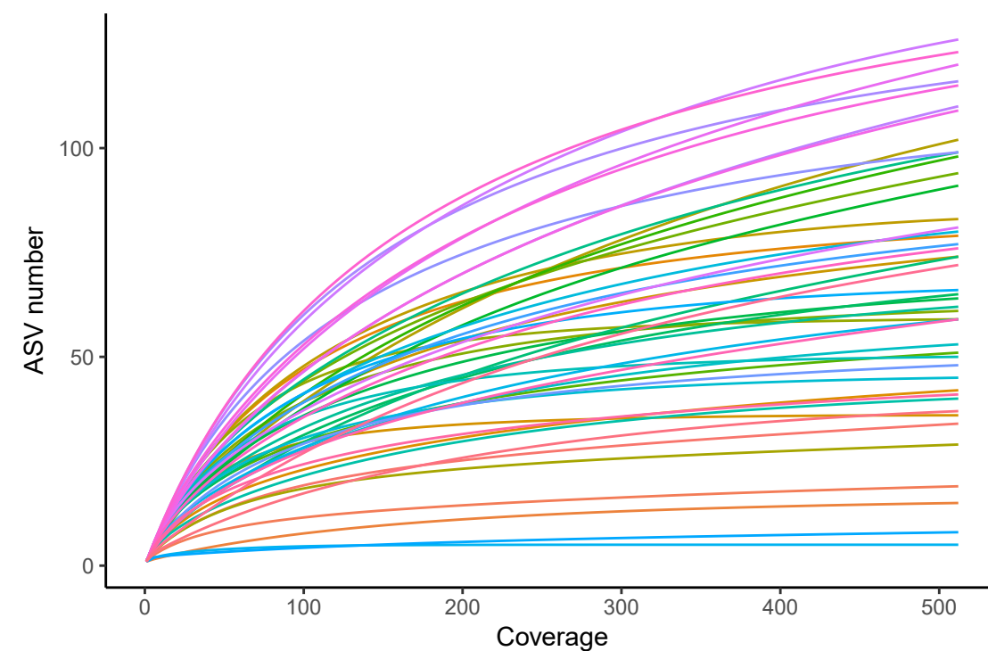
Rarefaction curve normalized root samples
