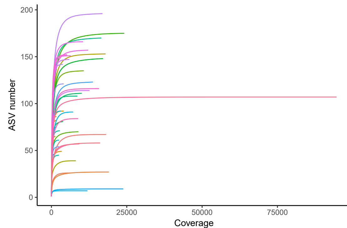
Rarefaction curve non-normalized root samples
