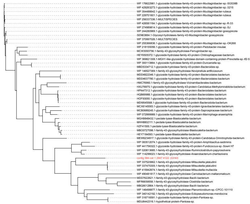
Fig S2. Maximum-likelihood phylogenetic tree of GH-43 proteins encoded by phage genomes and their closest reference homologs.
