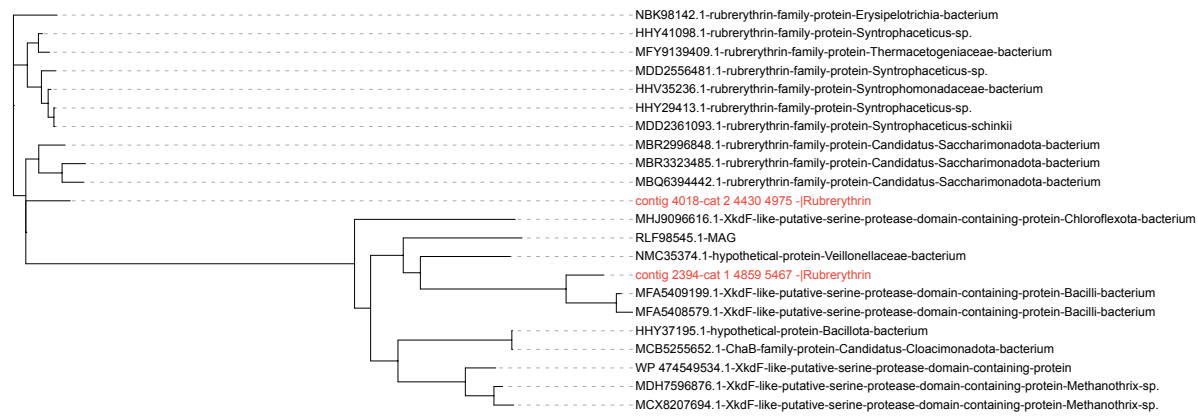
Fig S3. Maximum-likelihood phylogenetic tree of Rubrerythrin proteins encoded by phage genomes and their closest reference homologs.
