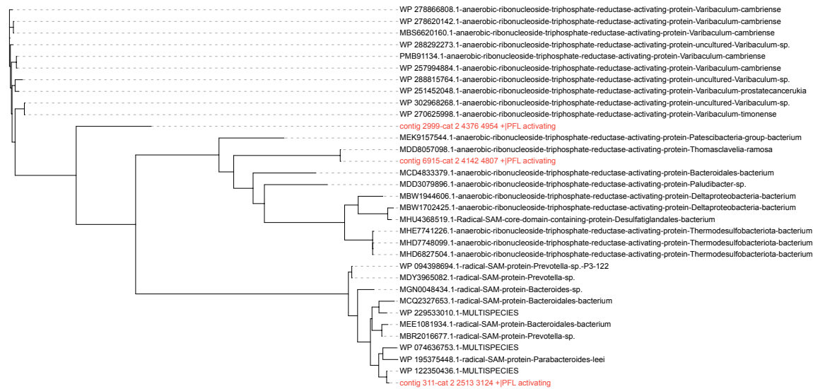
Fig S5. Maximum-likelihood phylogenetic tree of PFL Activating proteins encoded by phage genomes and their closest reference homologs.
