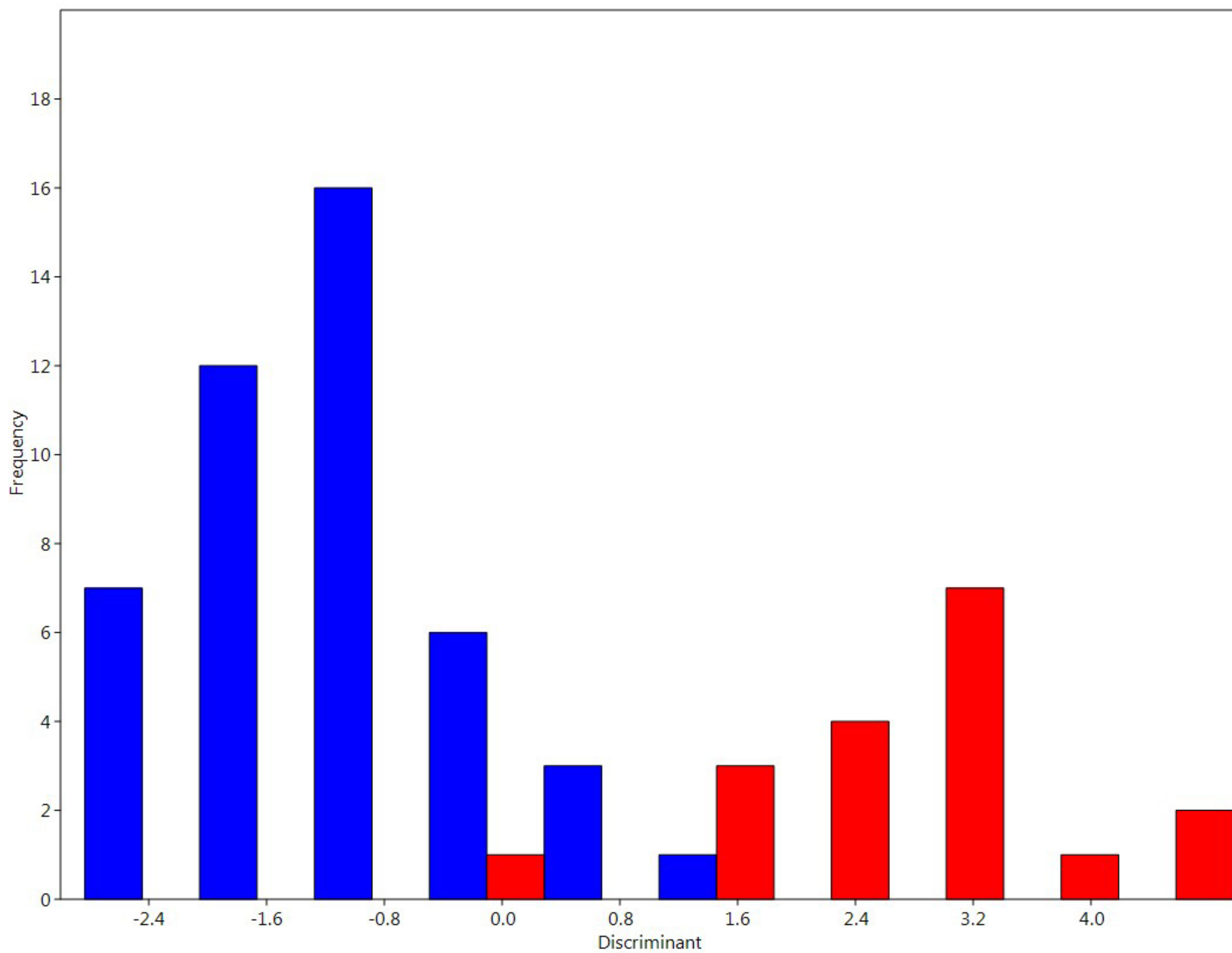
Figure S4: Histogram of results of discriminant analysis of C. lupaster (blue) and C. aureus (red).
