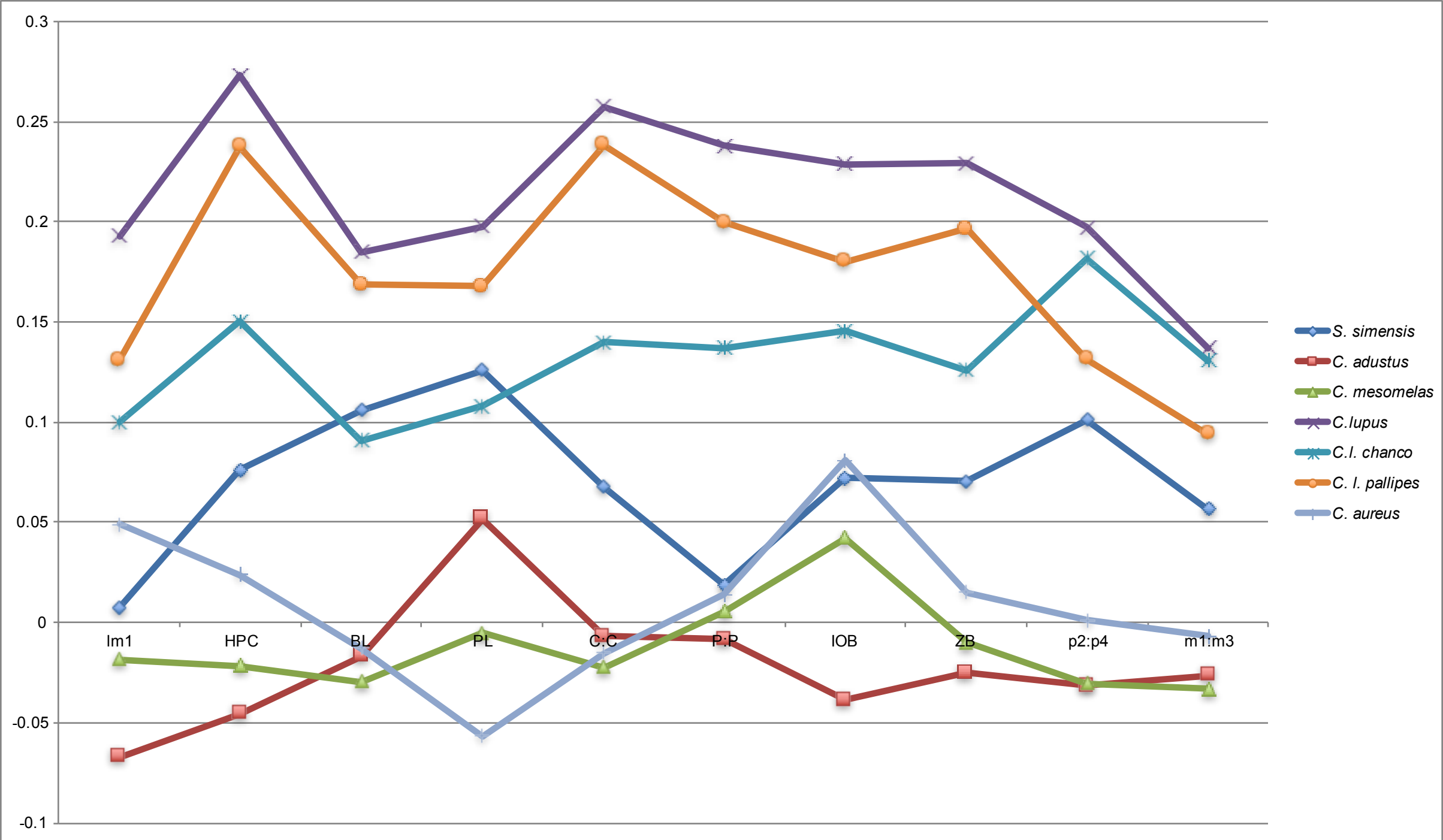
Figure S1: Ratio diagram of selected taxa and variables compared with C. lupaster (standard - all 0).
