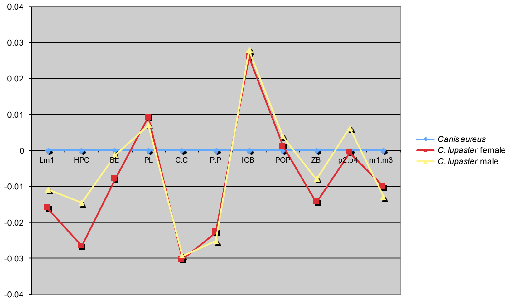
Figure S3: Ratio diagram comparing male and female C. lupaster to C. aureus (standard - all 0)
